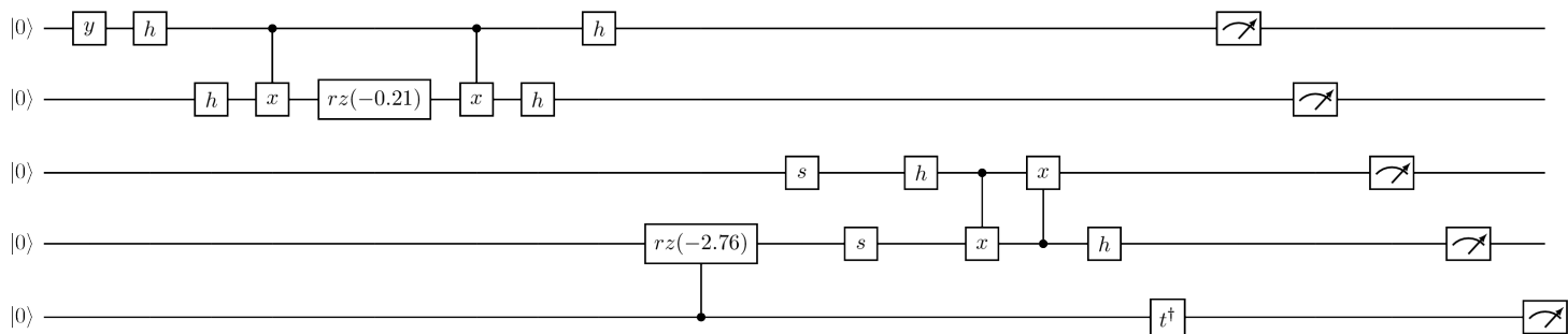
Figure 109: Tensor test 55 input
