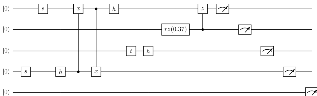
Figure 113: Tensor test 57 input
