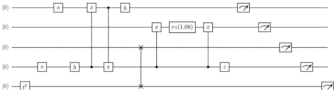
Figure 132: Tensor test66 output
