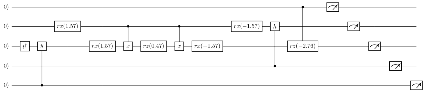
Figure 179: Tensor test 90 input
