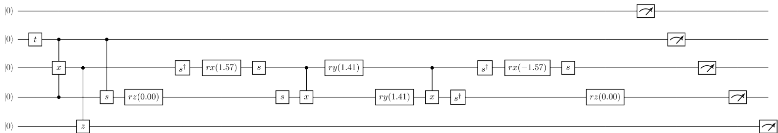
Figure 178: Tensor test 89 output
