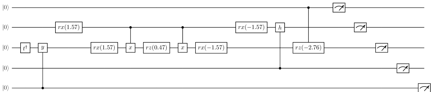
Figure 180: Tensor test 90 output
