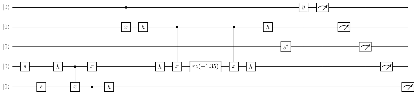
Figure 175: Tensor test 88 input
