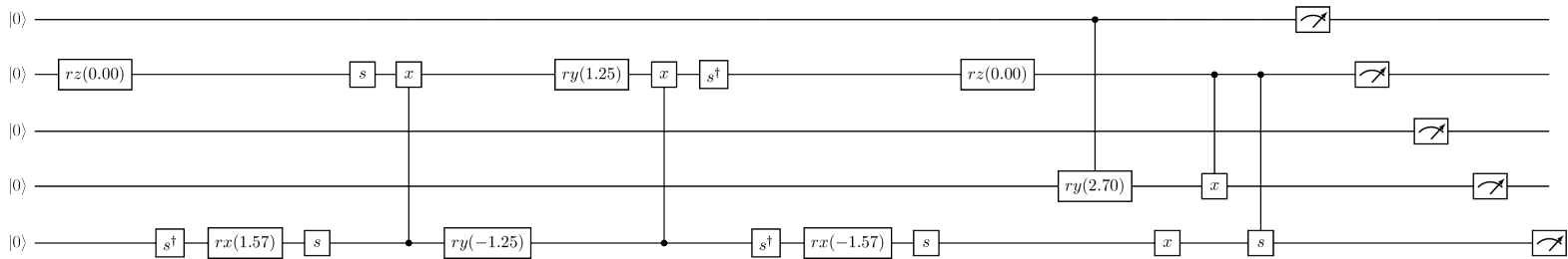
Figure 130: Tensor test65 output
