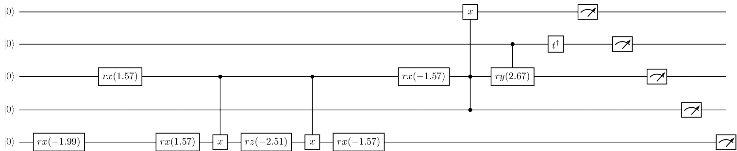
Figure 156: Tensor test 78 output
