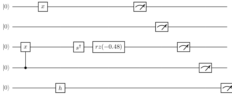
Figure 151: Tensor test 76 input
