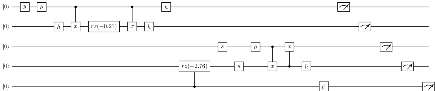
Figure 110: Tensor test 55 output
