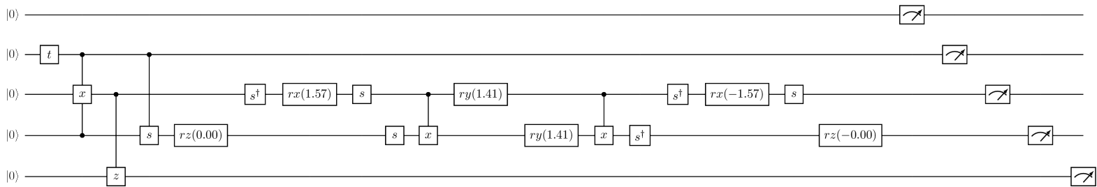
Figure 177: Tensor test 89 input
