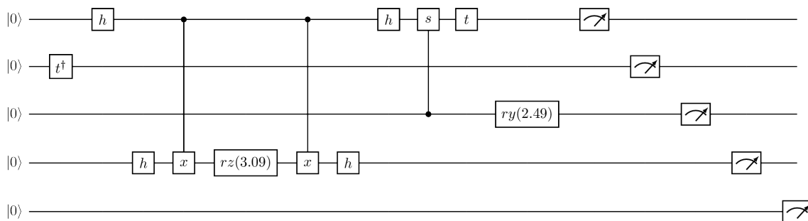
Figure 111: Tensor test 56 input
