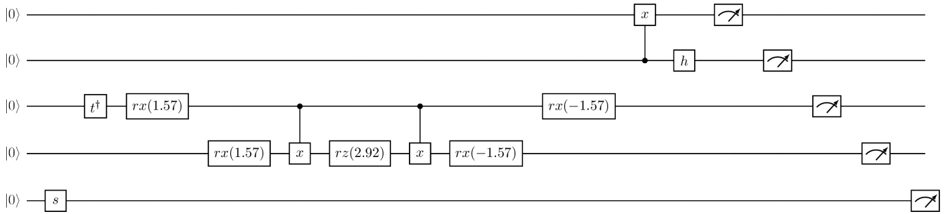
Figure 153: Tensor test 77 input
