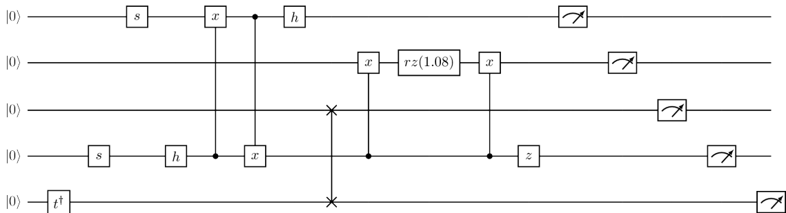
Figure 131: Tensor test66 input
