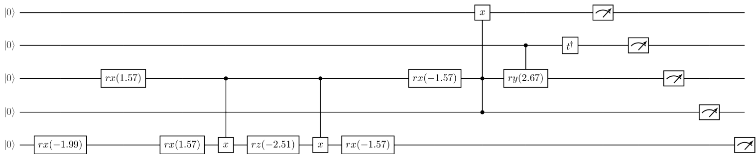
Figure 155: Tensor test 78 input
