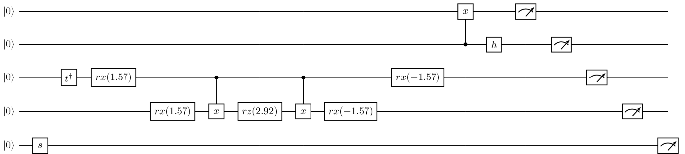
Figure 154: Tensor test 77 output
