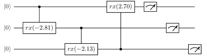
(b) HCrzHToCrx Output
