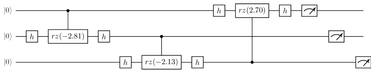
(a) HCrzHToCrx Input
