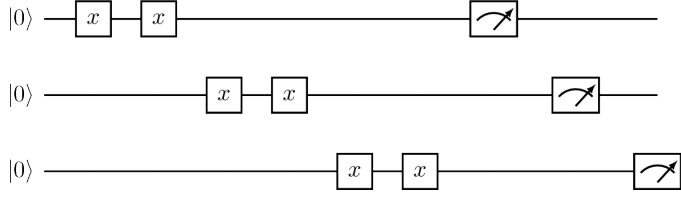
(a) XXToId Input
