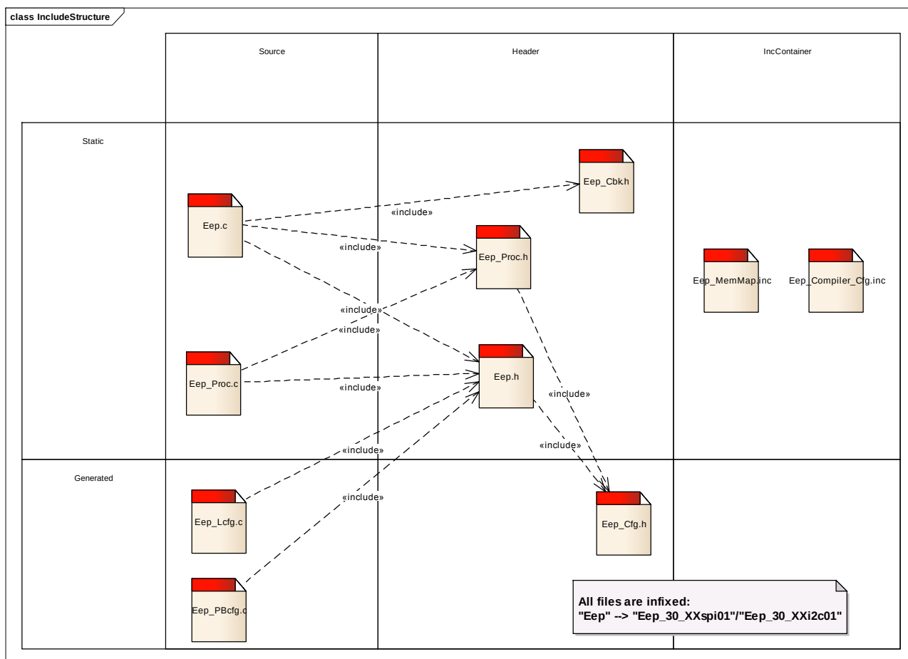
Figure 4-1 Include Structure
