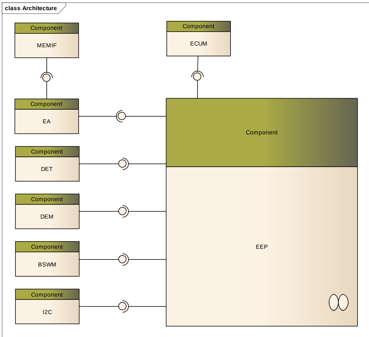
Figure 2-2 Interfaces to adjacent modules of the EEP
