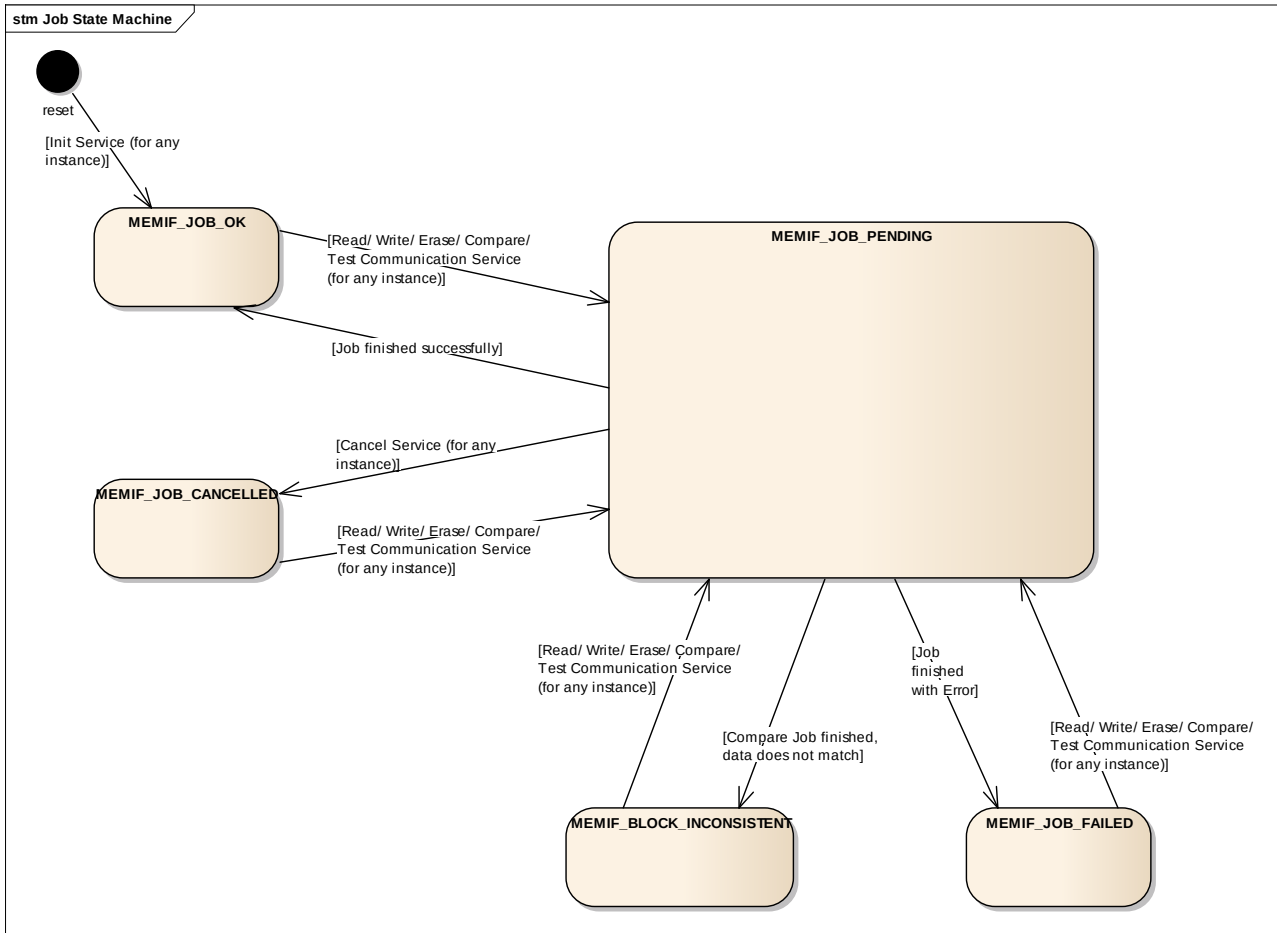
Figure 3-2 Job States
