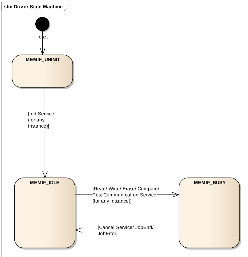
Figure 3-1 Module States
