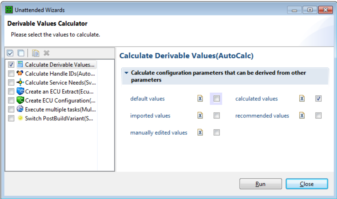
Figure 6.130. The Calculate Derivable Values wizard
