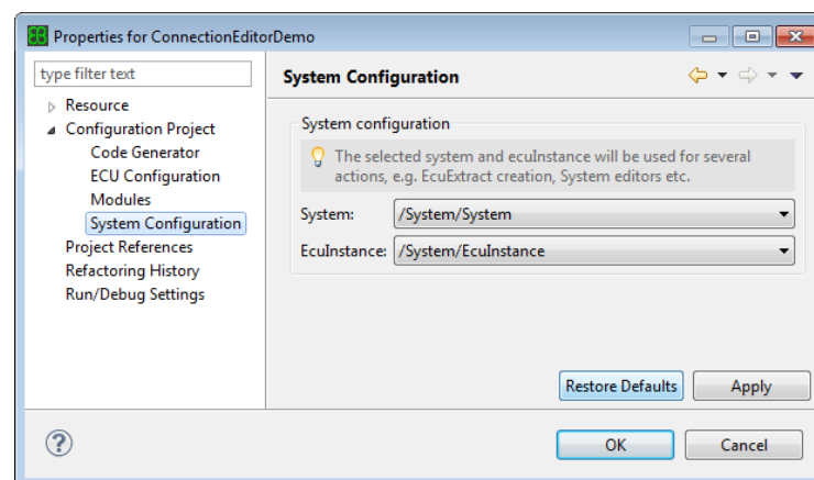
Figure 7.3. Setting the system and ECU instance
