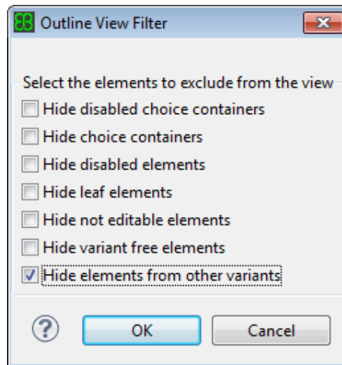
Figure 5.17. The Outline View Filter window
