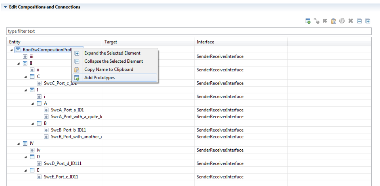
Figure 7.10. The Add Prototypes menu item
