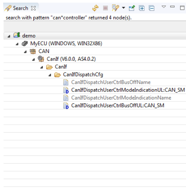
Figure 6.140. The Search view
