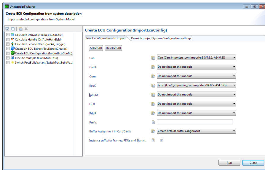
Figure 6.168. The Select configurations to import page
