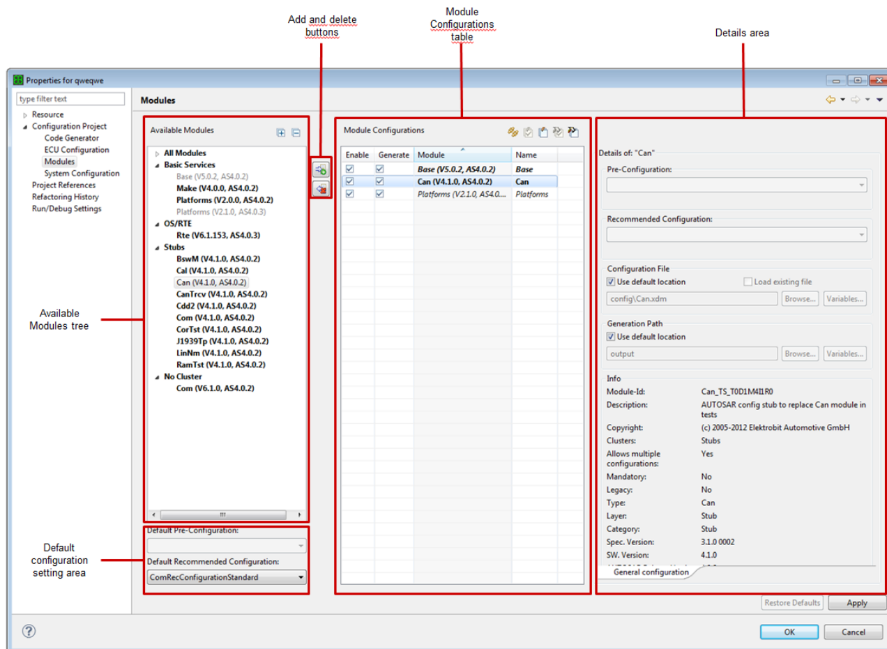
Figure 6.23. Editing module configurations on the Modules page of the project properties
