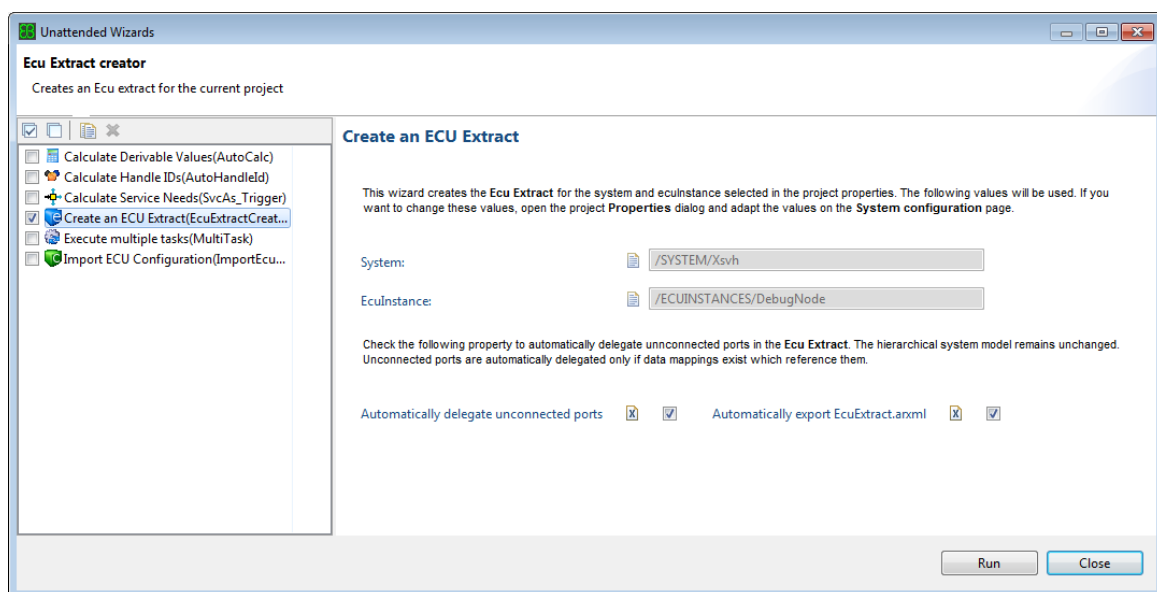
Figure 6.170. Unattended wizard for ECU Extract creation
