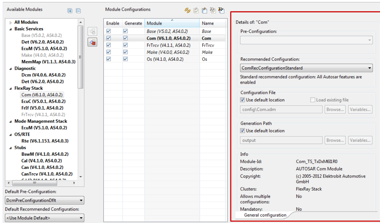
Figure 6.100. The Details area in the Module Configurations page
