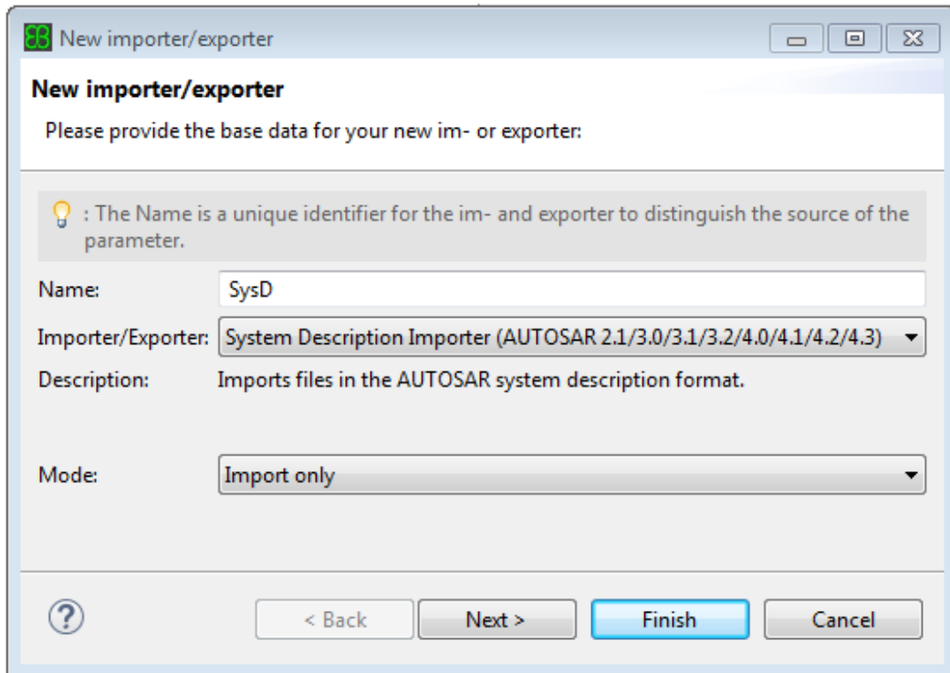
Figure 6.153. The New Importer/Exporter dialog
