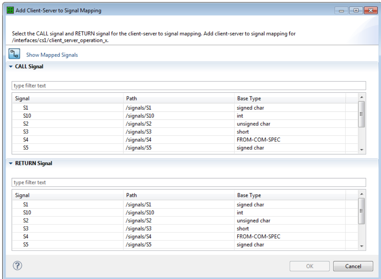
Figure 7.27. The Add Client-Server to Signal Mapping dialog
