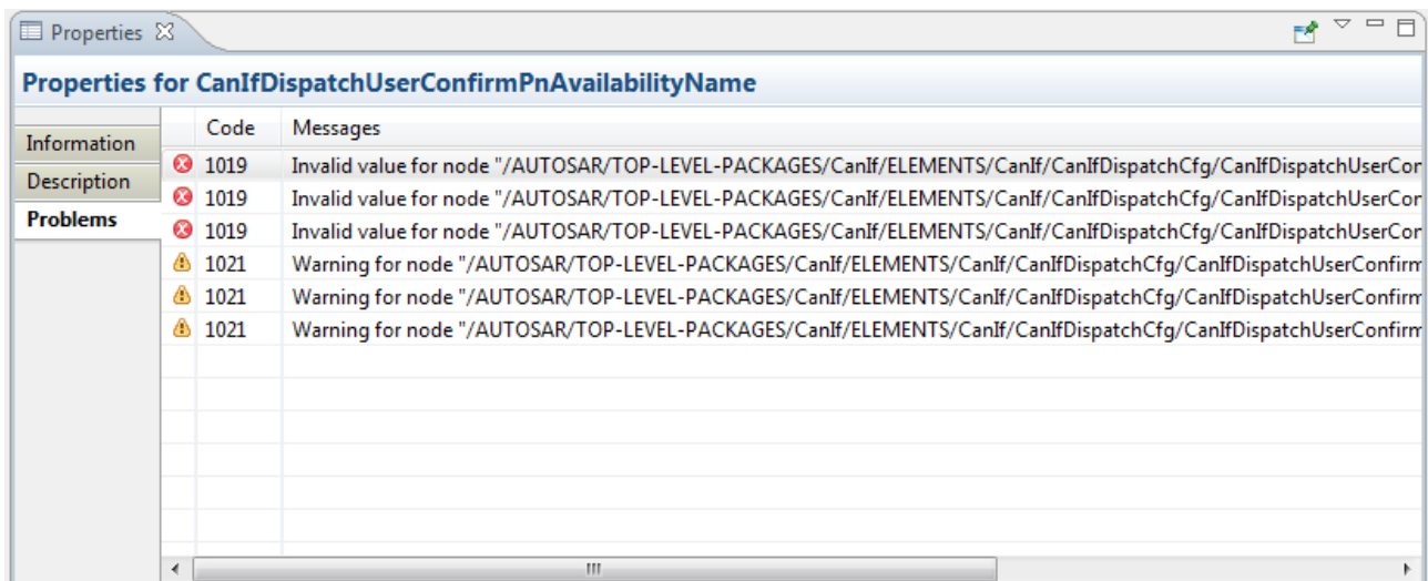
Figure 5.31. The Problems tab
