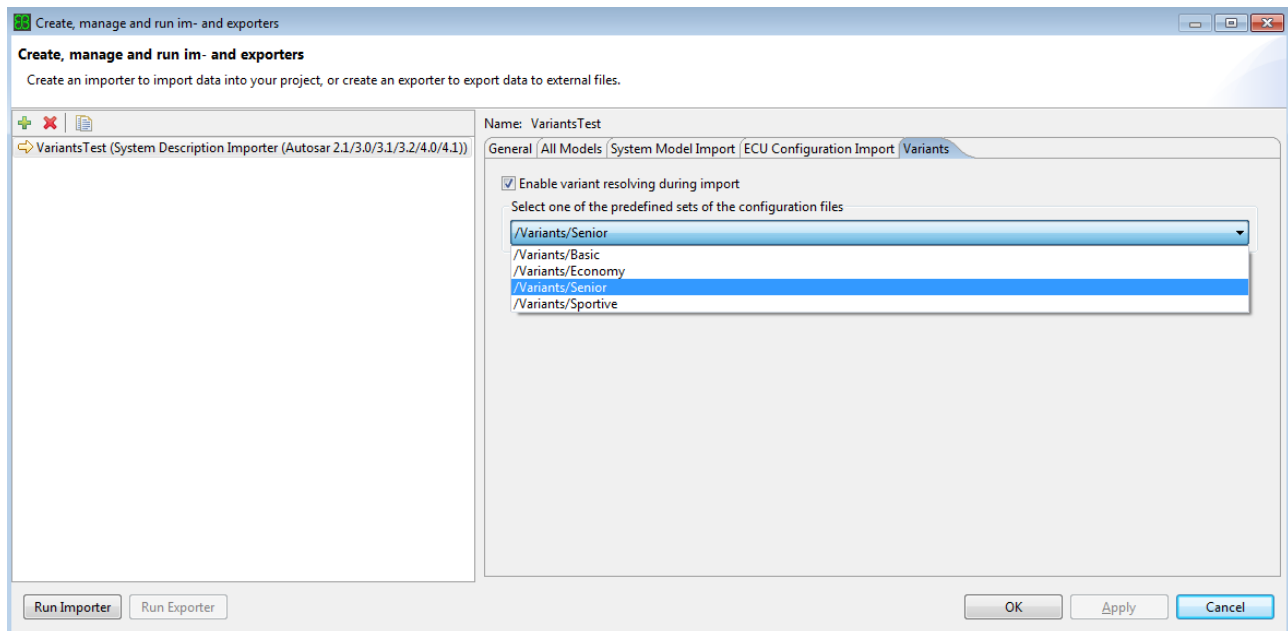
Figure 6.157. The Variants tab
