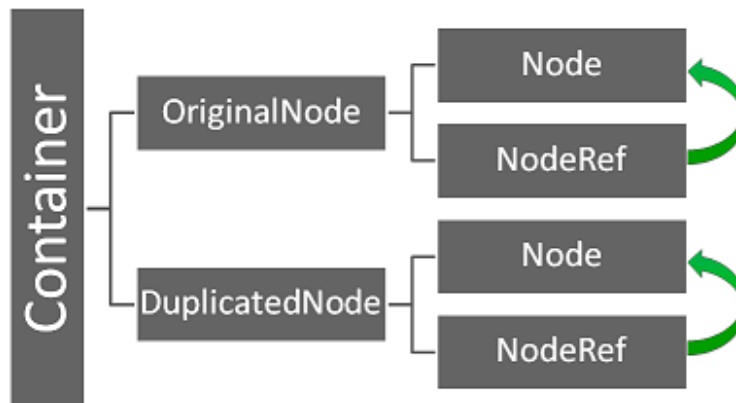
Figure 5.42. Duplicating elements with references
