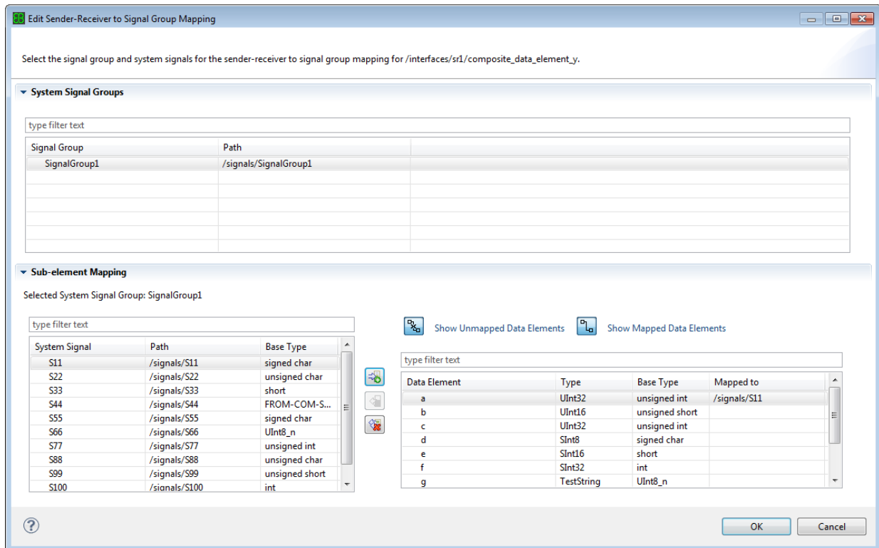
Figure 7.29. The Edit Sender-Receiver to Signal Group Mapping dialog
