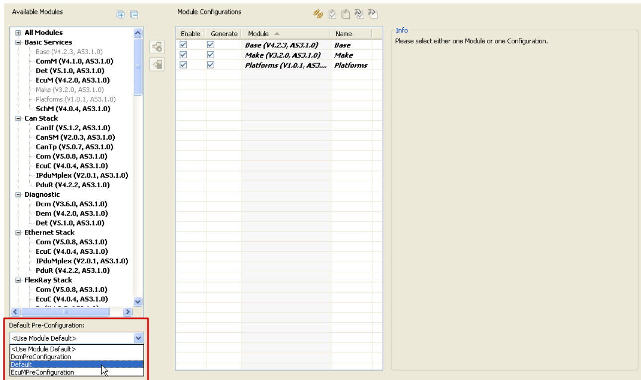
Figure 6.32. Selecting the default preconfiguration for new module configurations
