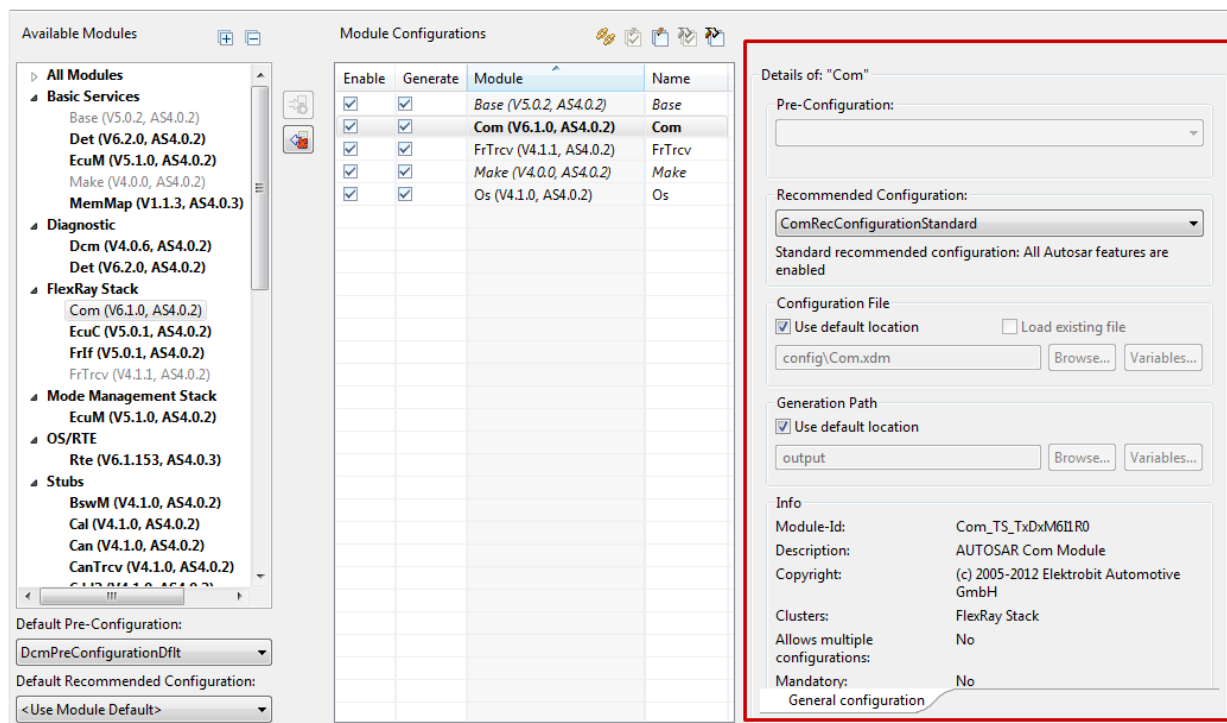
Figure 6.97. The Details area in the Module Configurations page
