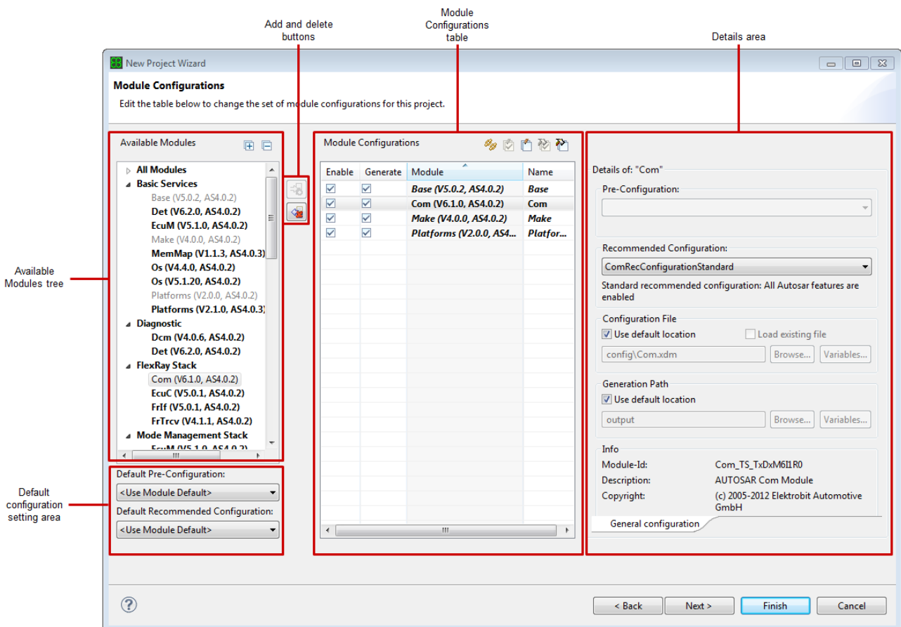
Figure 6.3. The Module Configurations page
