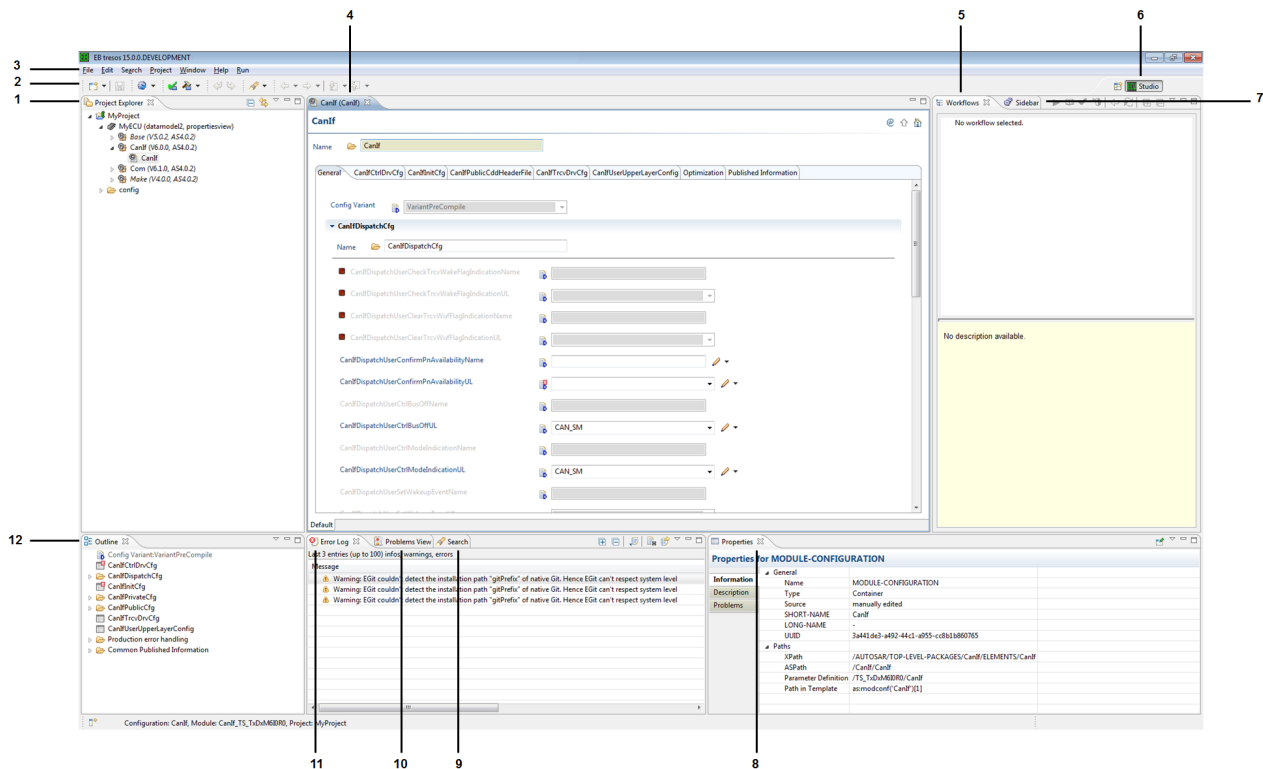
Figure 5.1. The EB tresos Studio Workbench
