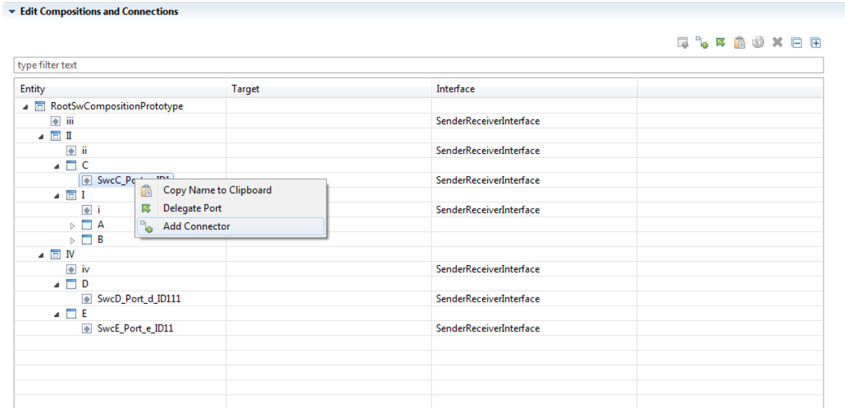
Figure 7.7. The Add Connector menu item
