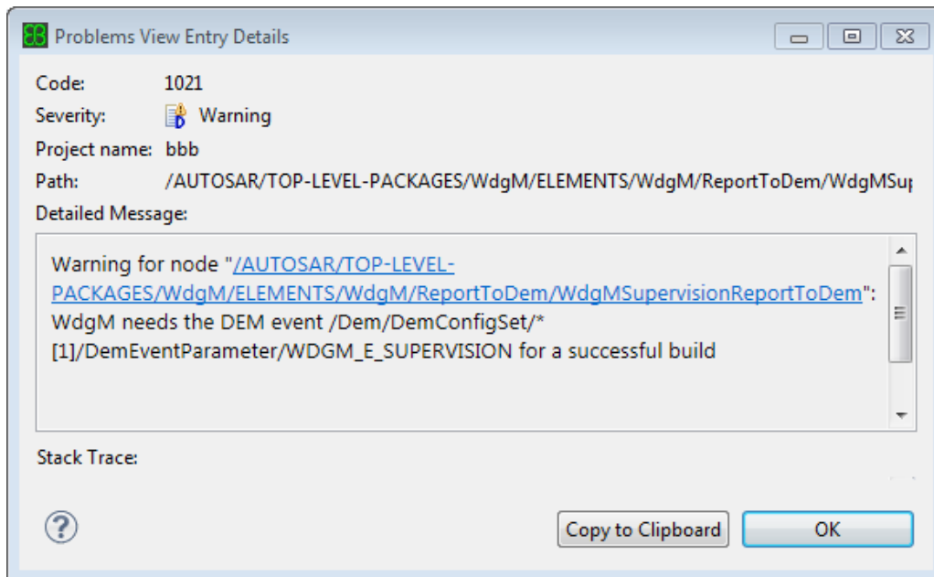
Figure 5.20. Details of the Problems View view
