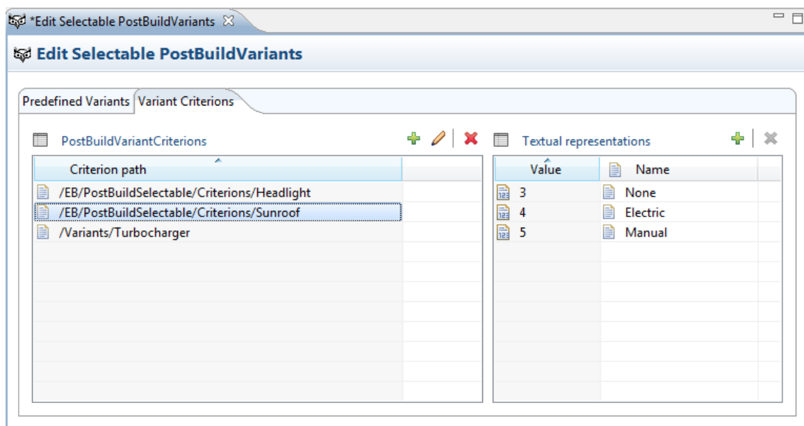
Figure 7.34. The Variant Criteria page
