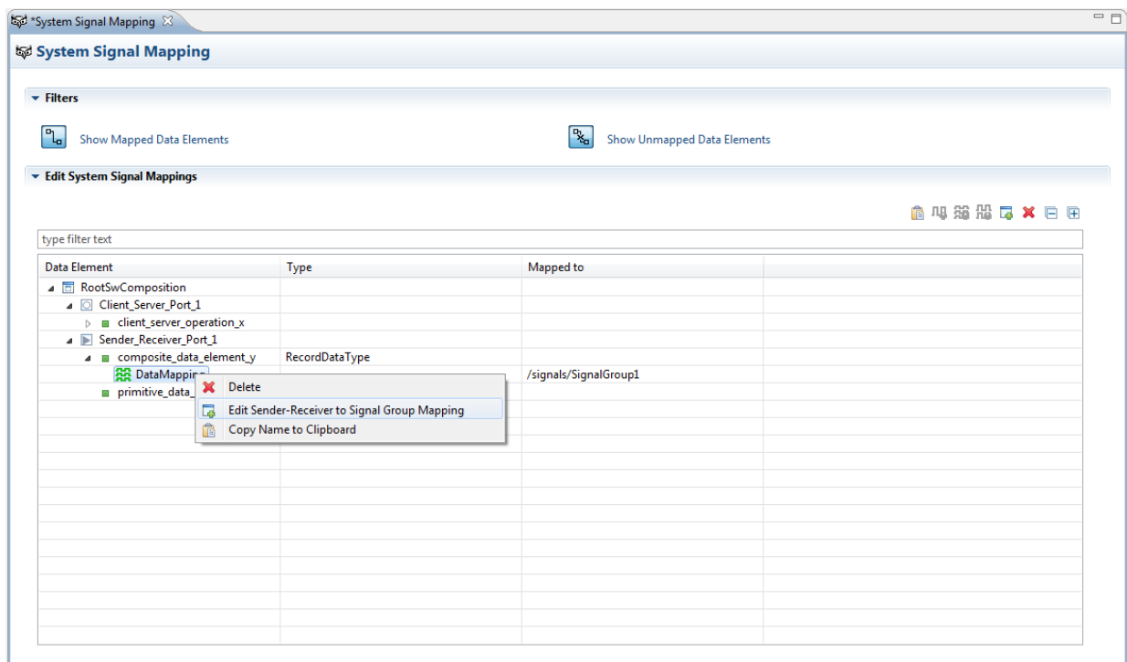
Figure 7.28. The Edit Sender-Receiver to Signal Group Mapping menu item
