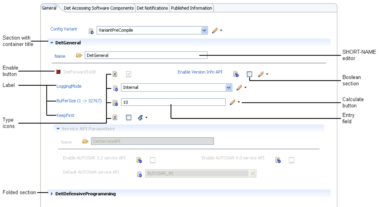
Figure 5.36. The GUI elements of the Generic Configuration Editor: sections, labels, type icons
