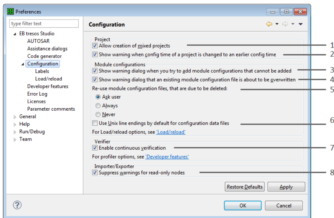
Figure 6.1. Preferences subpage Configuration
