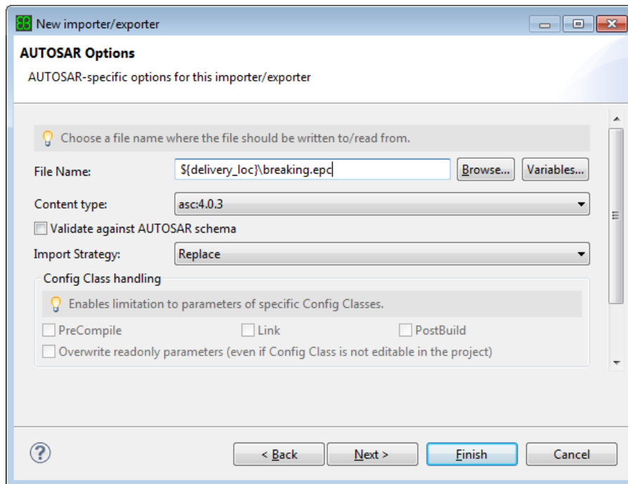
Figure 6.152. AUTOSAR importer using path variable
