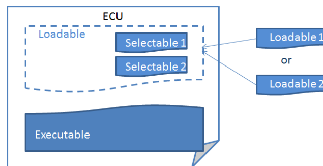
Figure 6.175. Combined loadable and selectable concept
