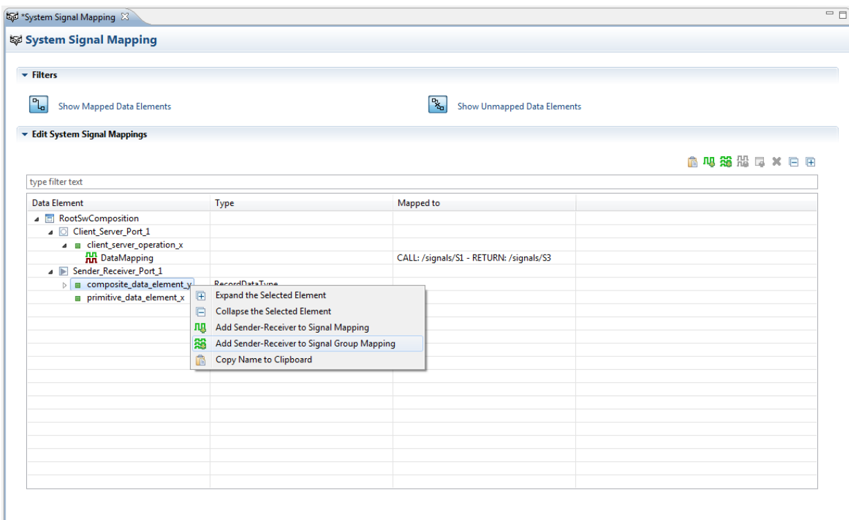
Figure 7.24. The Add Sender-Receiver to Signal Group Mapping menu item
