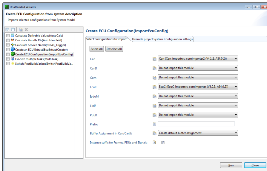
Figure 6.165. The unattended wizard to Create ECU Configuration
