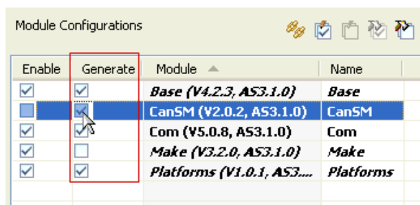
Figure 6.9. Enabling code generation for one module configuration
