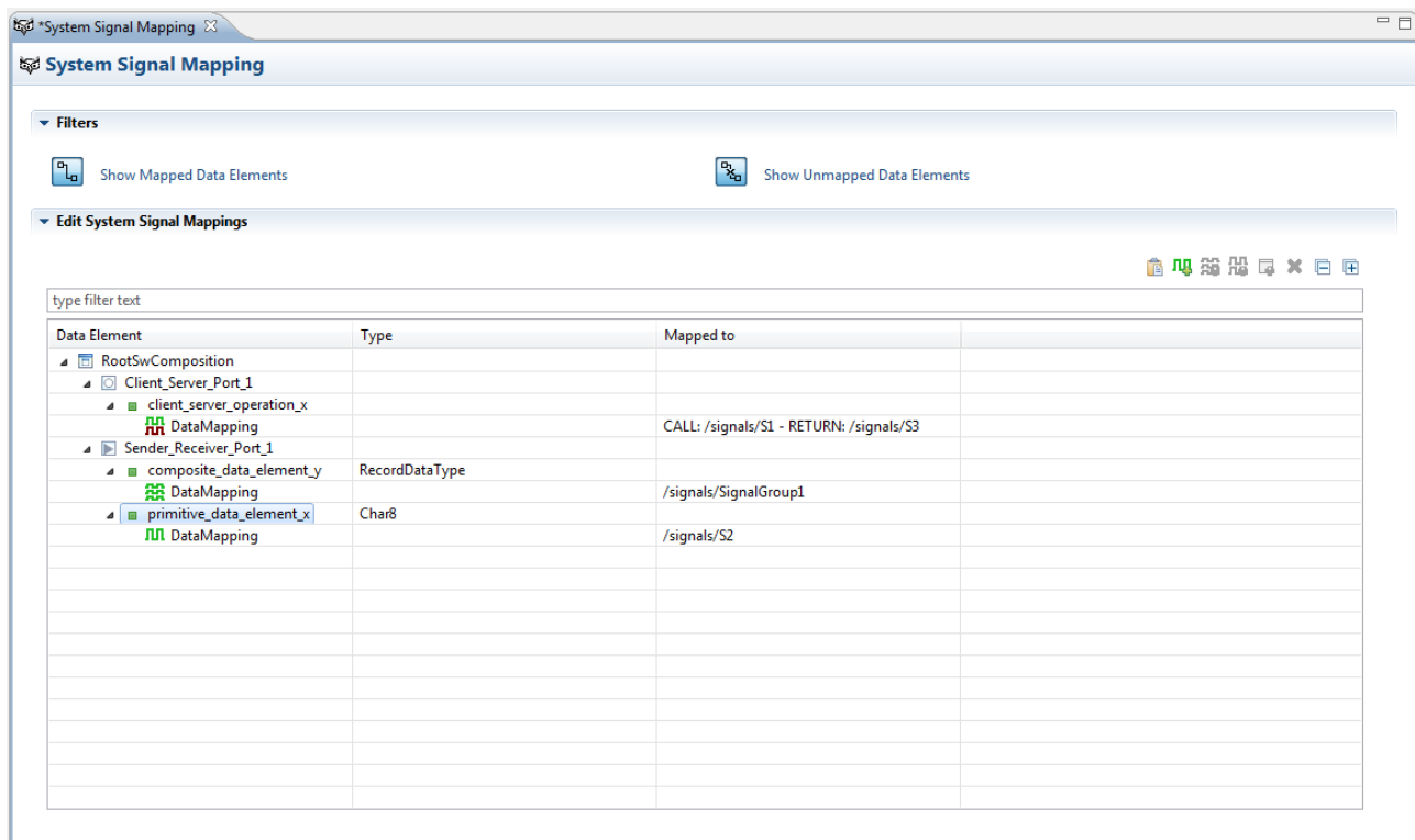
Figure 7.18. Data mappings are displayed as children of the ports
