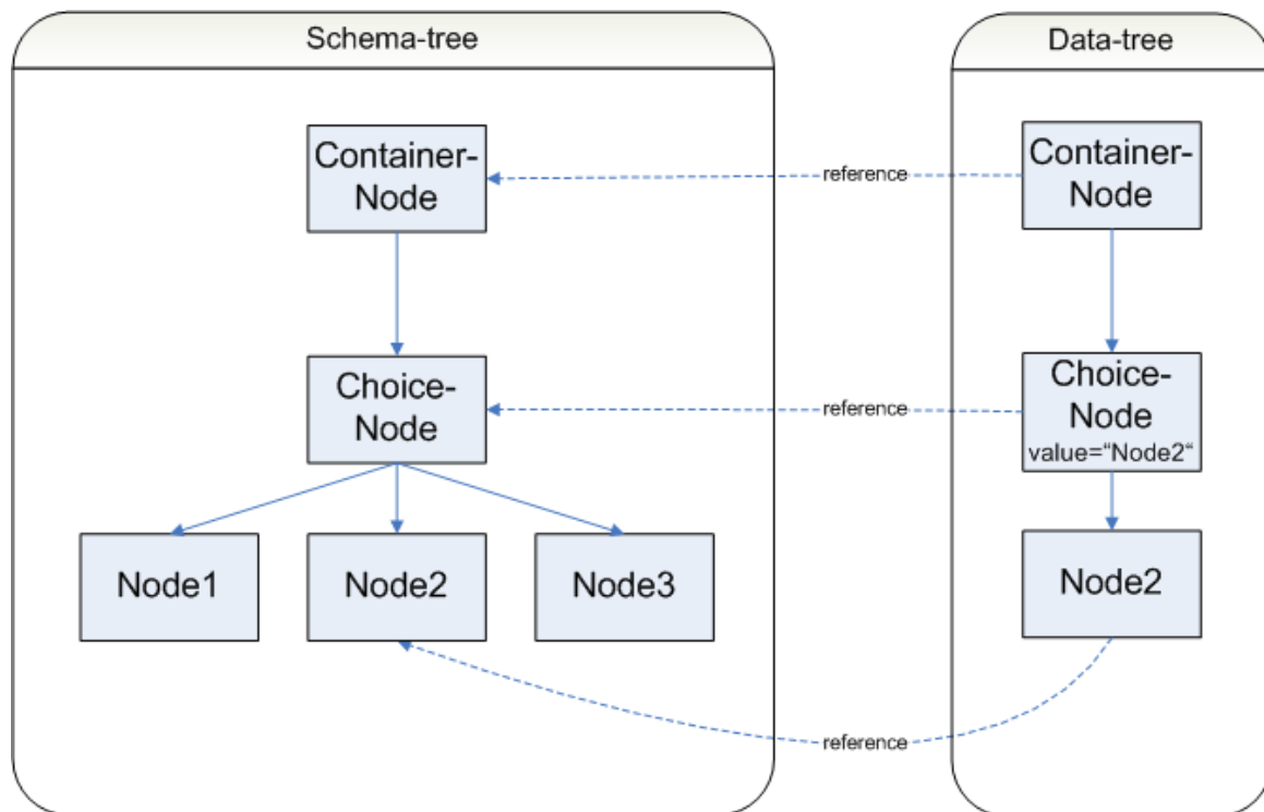
Figure 6.7. Choice-Representation
