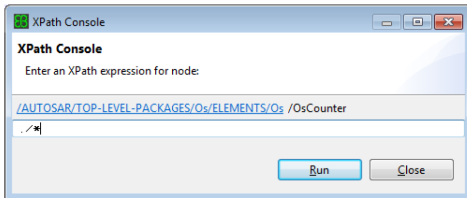
Figure 6.59. XPath Console
