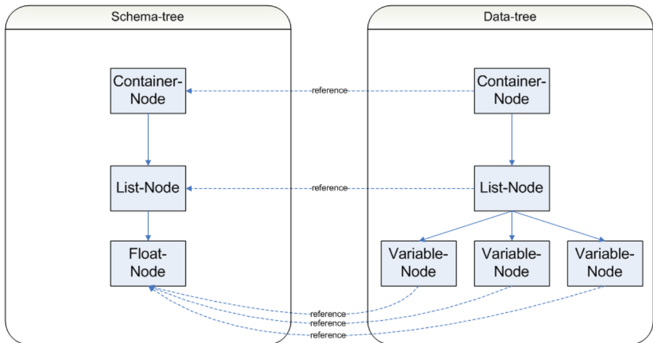
Figure 6.6. List-Representation
