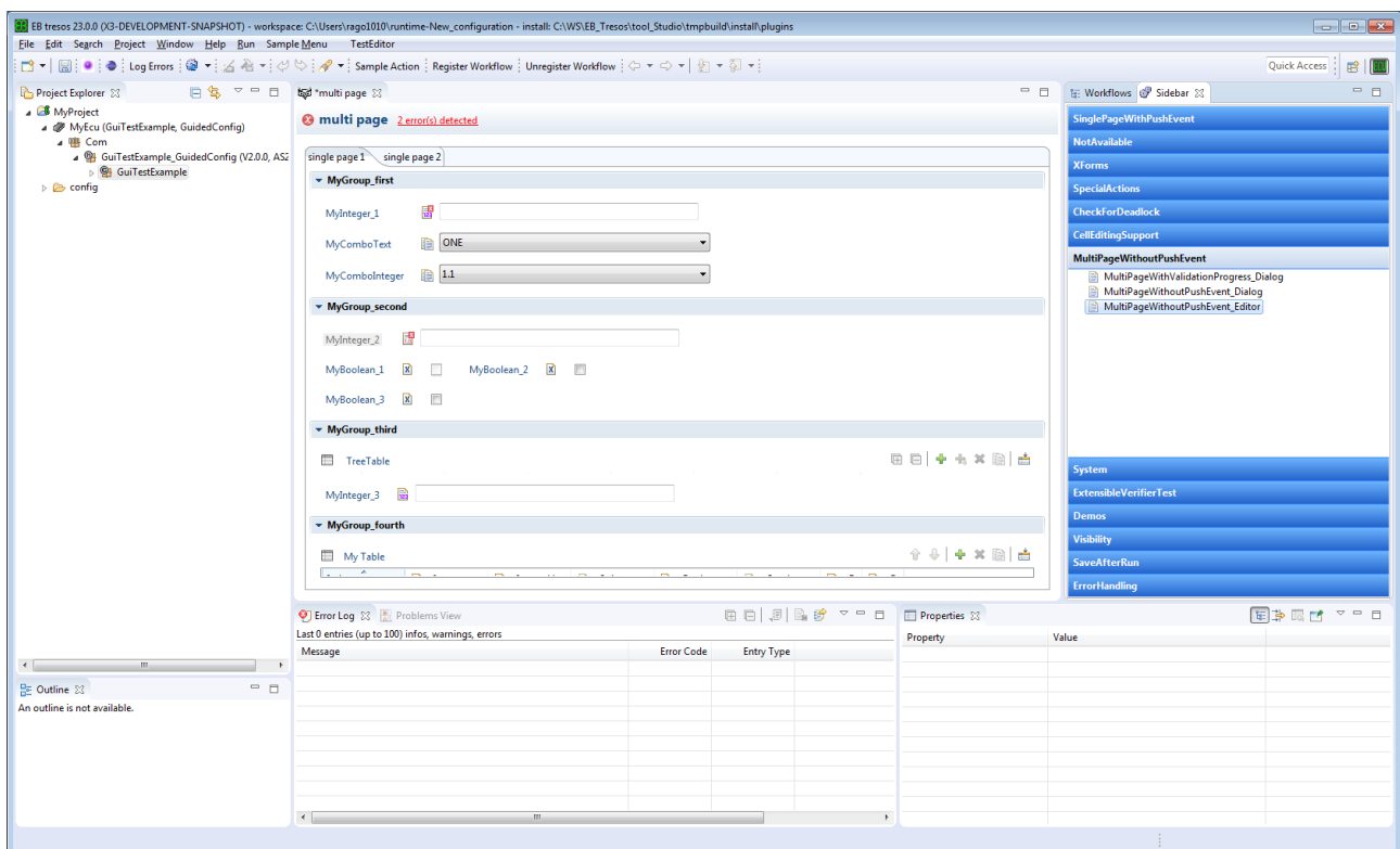
Figure 8.5. Standalone editor
