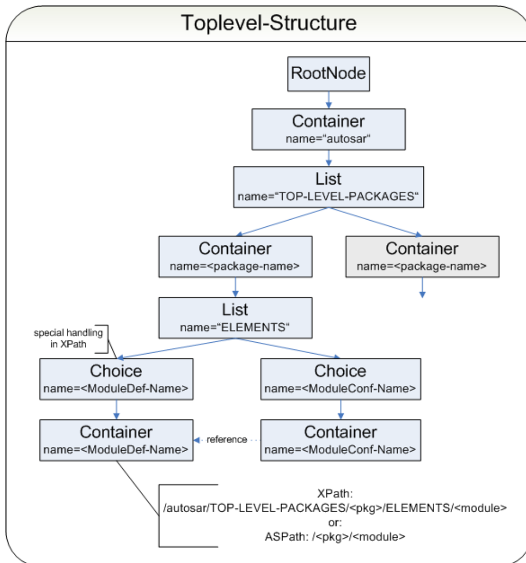
Figure 5.4. Top level structure for AUTOSAR-nodes
