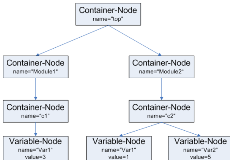
Figure 6.61. Example-Tree
