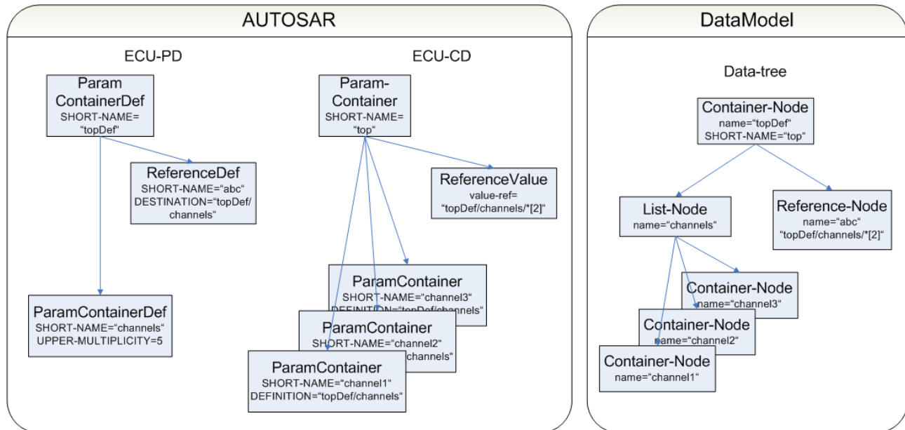
Figure 5.7. Reference-Example
