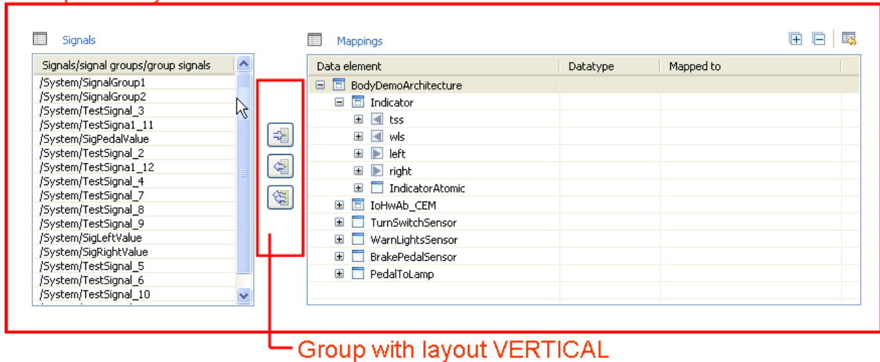
Figure 8.12. Example layout
