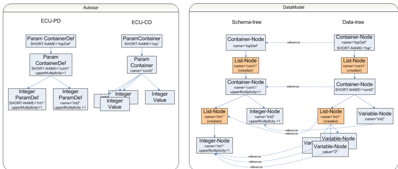
Figure 5.5. List-Representation
