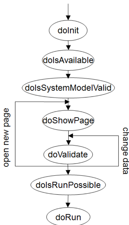
Figure 8.11. Wizard lifecycle
