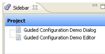
Figure 8.52. Sidebar view
