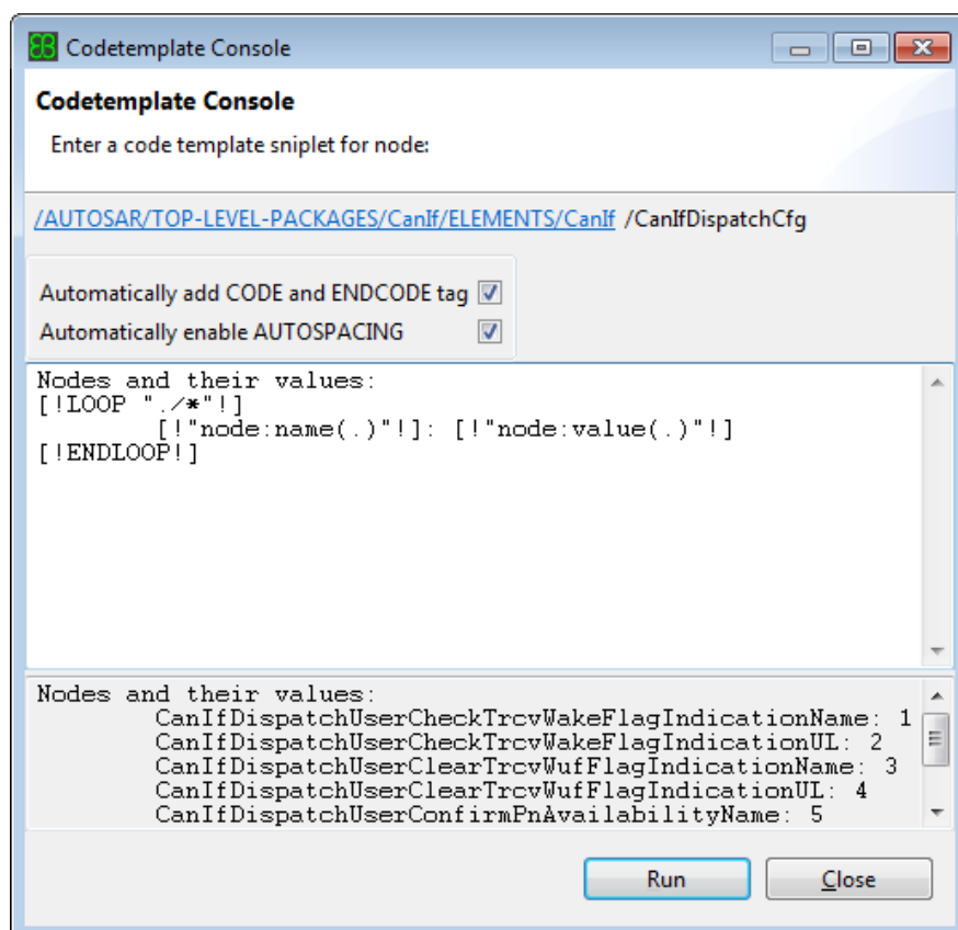
Figure 7.3. Codetemplate console
