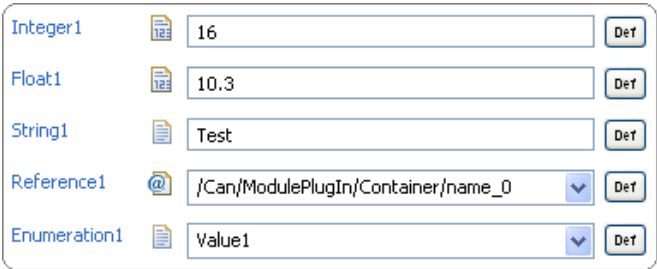
Figure 6.19. Field elements
