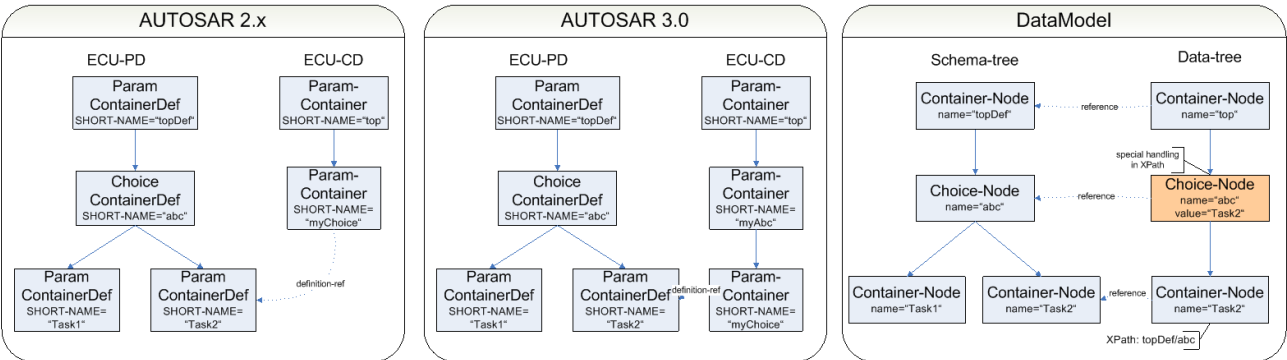
Figure 5.6. Choice-Representation
