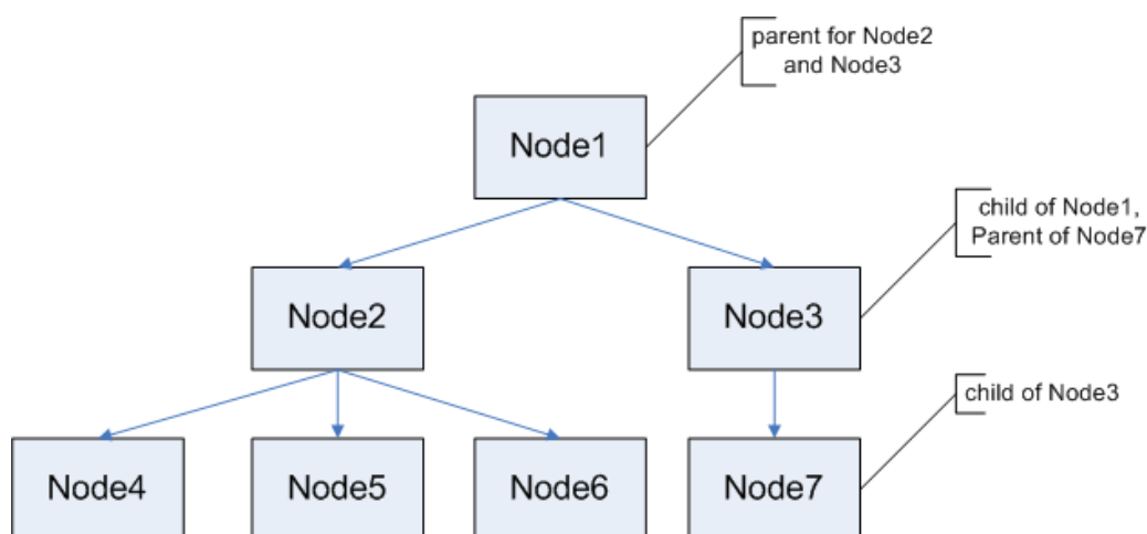
Figure 6.1. Simple Node-Tree
