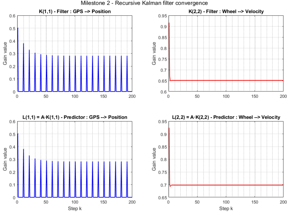
Figure 6: Convergence of the time-varying Kalman gain L_{\text{rec}}(k) = AK(k) (predictor form) to its periodic steady state, starting from an initial covariance P(0) = I_3 . Each panel shows one entry of the 3 \times 2 gain matrix. The recursive gain becomes periodic with period N = 10 after a brief transient, converging toward the offline LMI gain values. The residual gap \Delta_k between these two approaches is quantitatively analyzed in Section 5.3.
