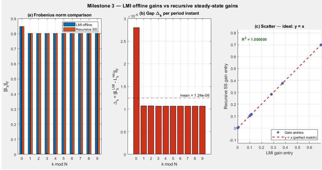
Figure 7: Quantitative comparison between the offline LMI gains L_k and the recursive steady-state gains L_{rec,ss}(k) (predictor form). Panel (a) shows Frobenius norms; panel (b) shows the entry-wise gap \Delta_k ; panel (c) shows the scatter plot of all entries against the identity line. The gap \Delta_k is of order 10^{-6} across all instants, lying within numerical solver tolerances and confirming that the LMI bound is tight for this system.
