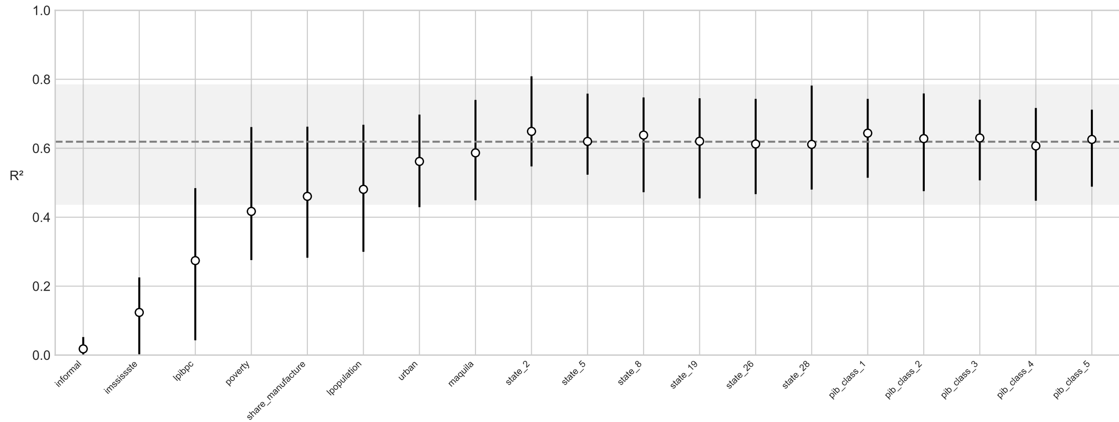
V4b: Importancia de variables — Outcome nuisance (BART Normal)
