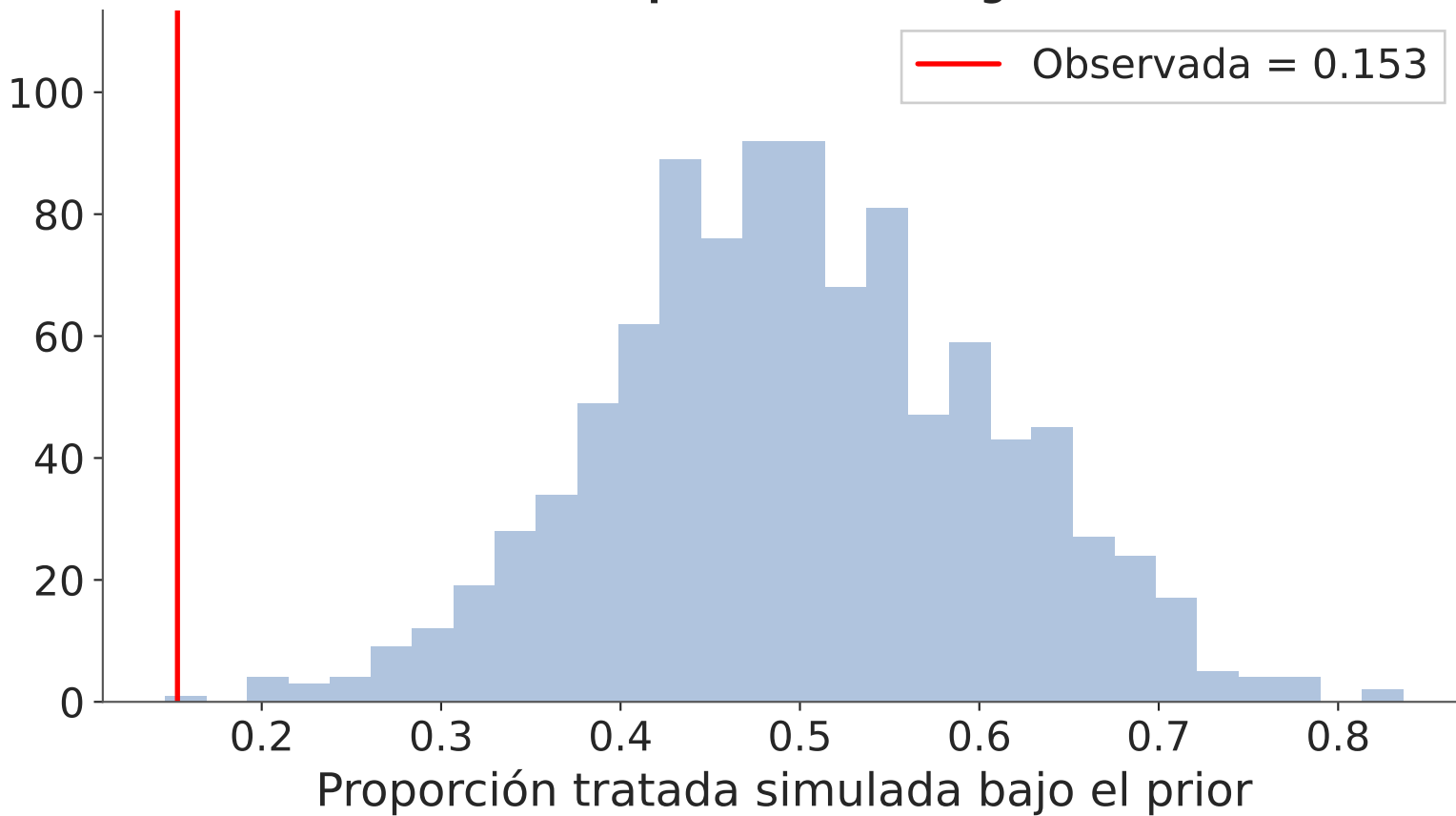
Prior predictive — Logit
