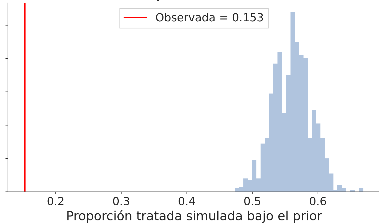
Prior predictive — BART
