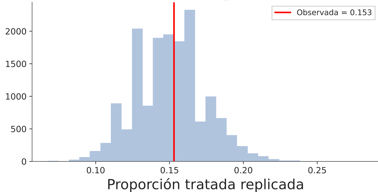
Global — BART ( p_B = 0.459 )
