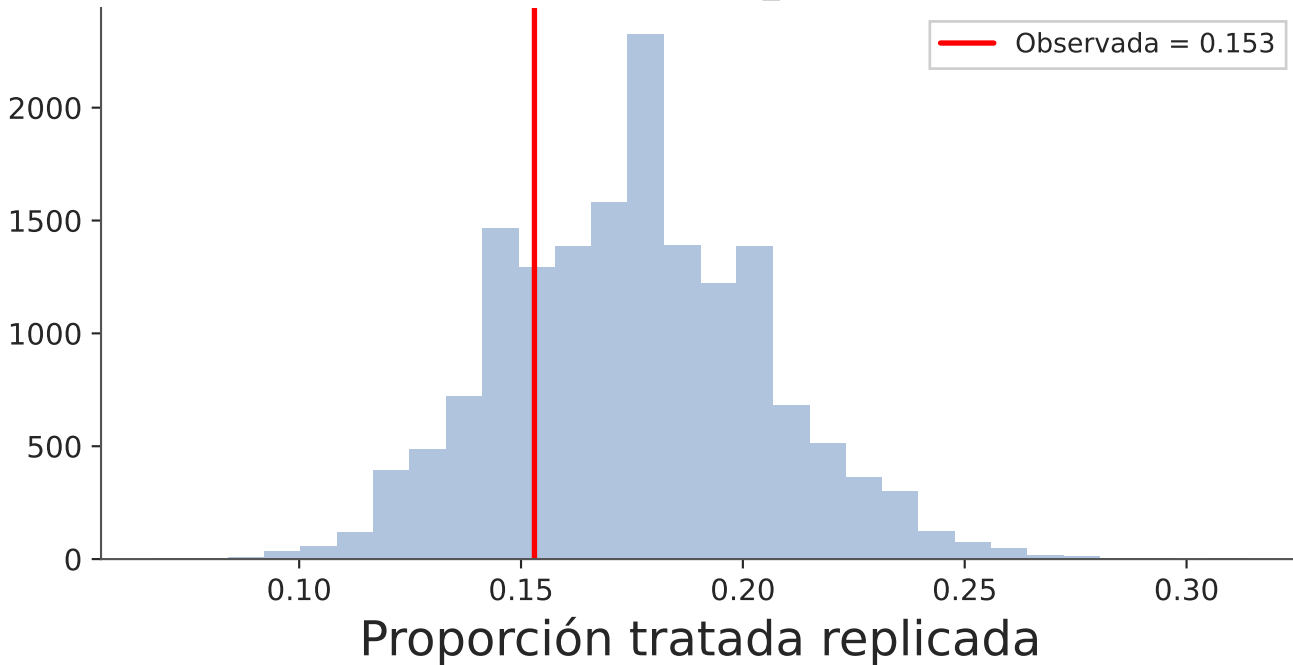
Global — Logit ( p_B = 0.794 )
