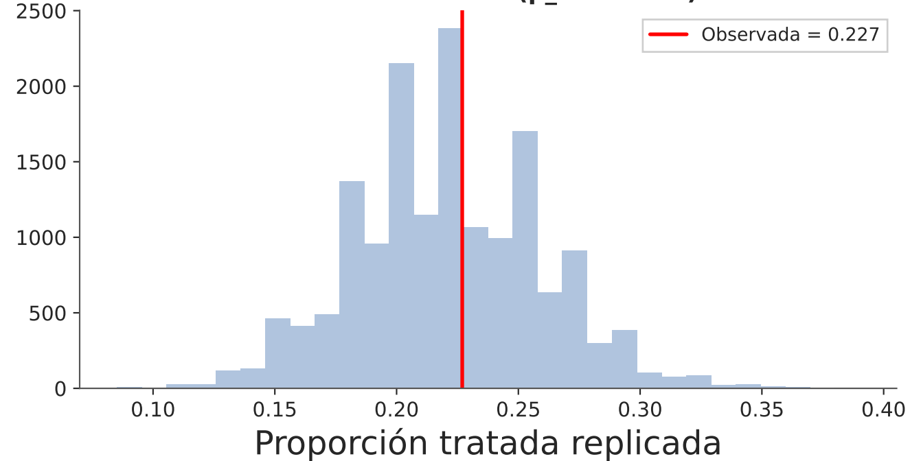
Urbanos — BART ( p_B = 0.467 )
