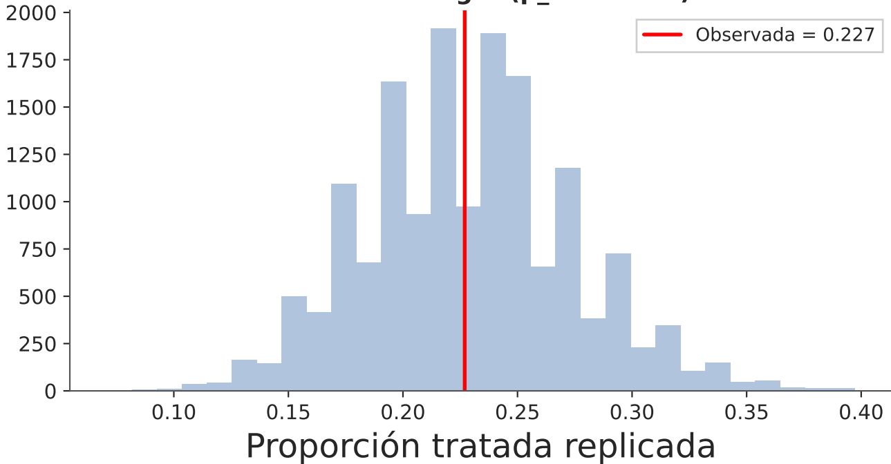
Urbanos — Logit ( p_B = 0.527 )
