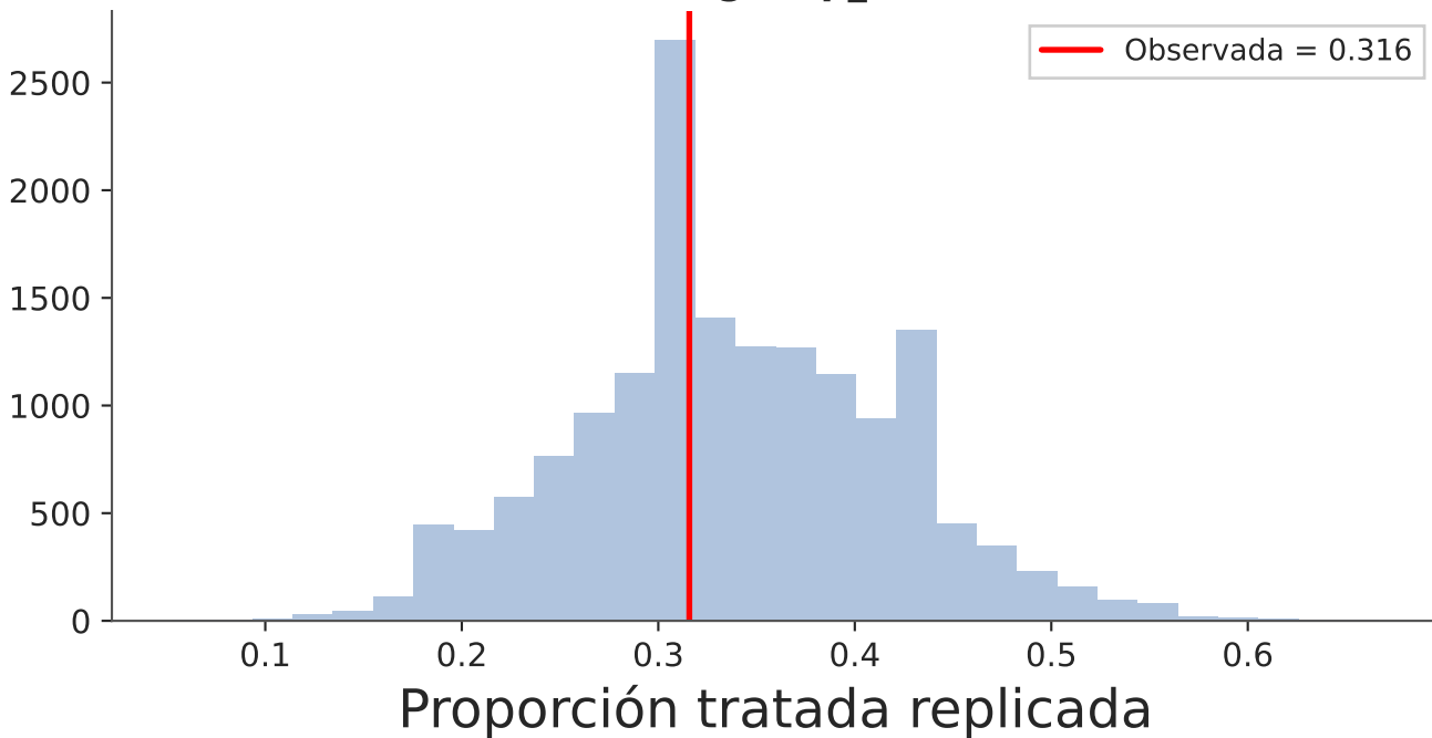
PIB Q5 — Logit ( p_B = 0.636 )
