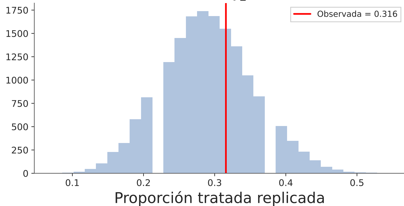
PIB Q5 — BART ( p_B = 0.384 )
