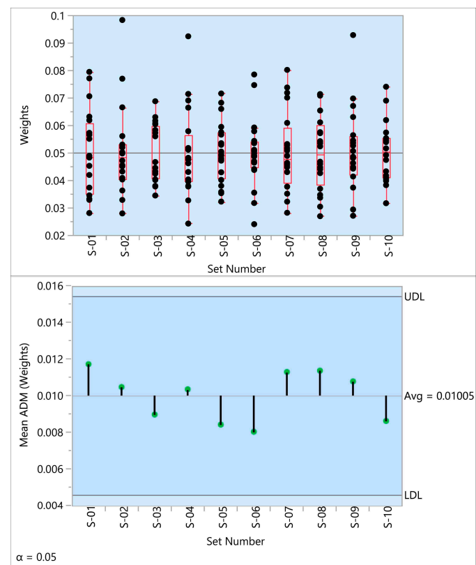
Figure 6. The results of ANOM for variances for category (iii).
