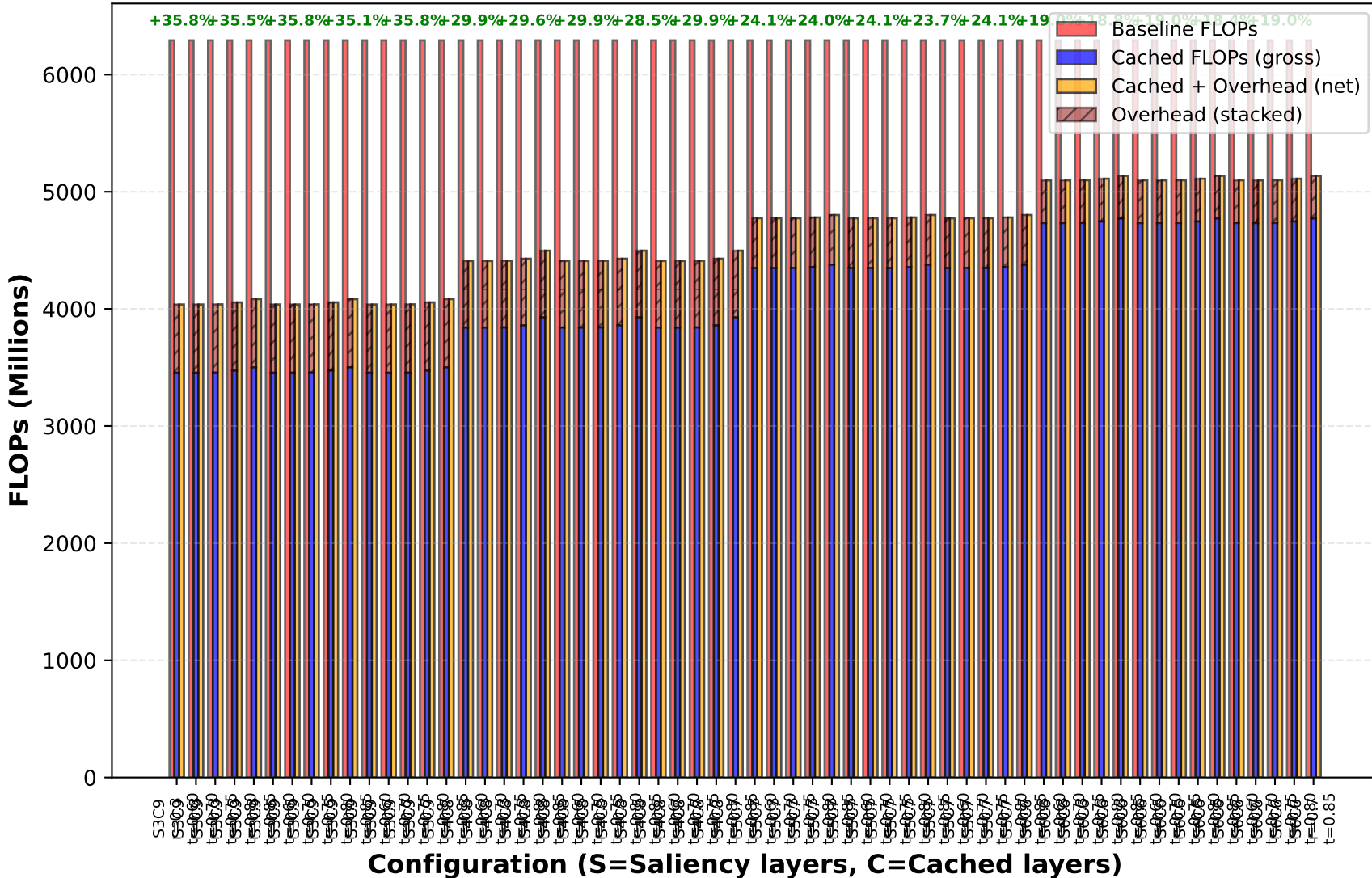
FLOP Comparison: Baseline vs Cached vs Overhead
