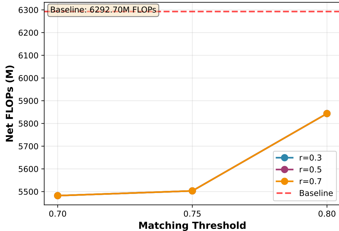
FLOPs vs Threshold (saliency=4)
