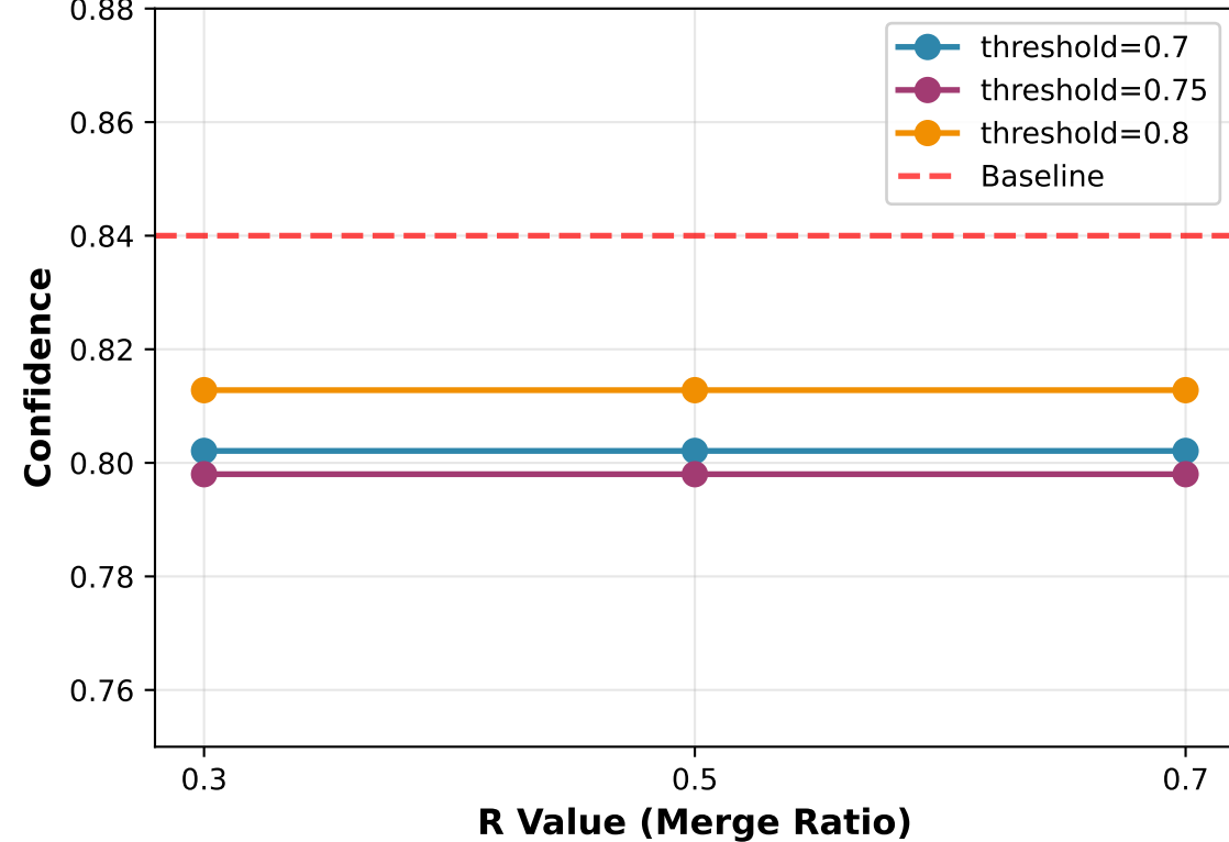
Confidence vs R Value (saliency=4)
