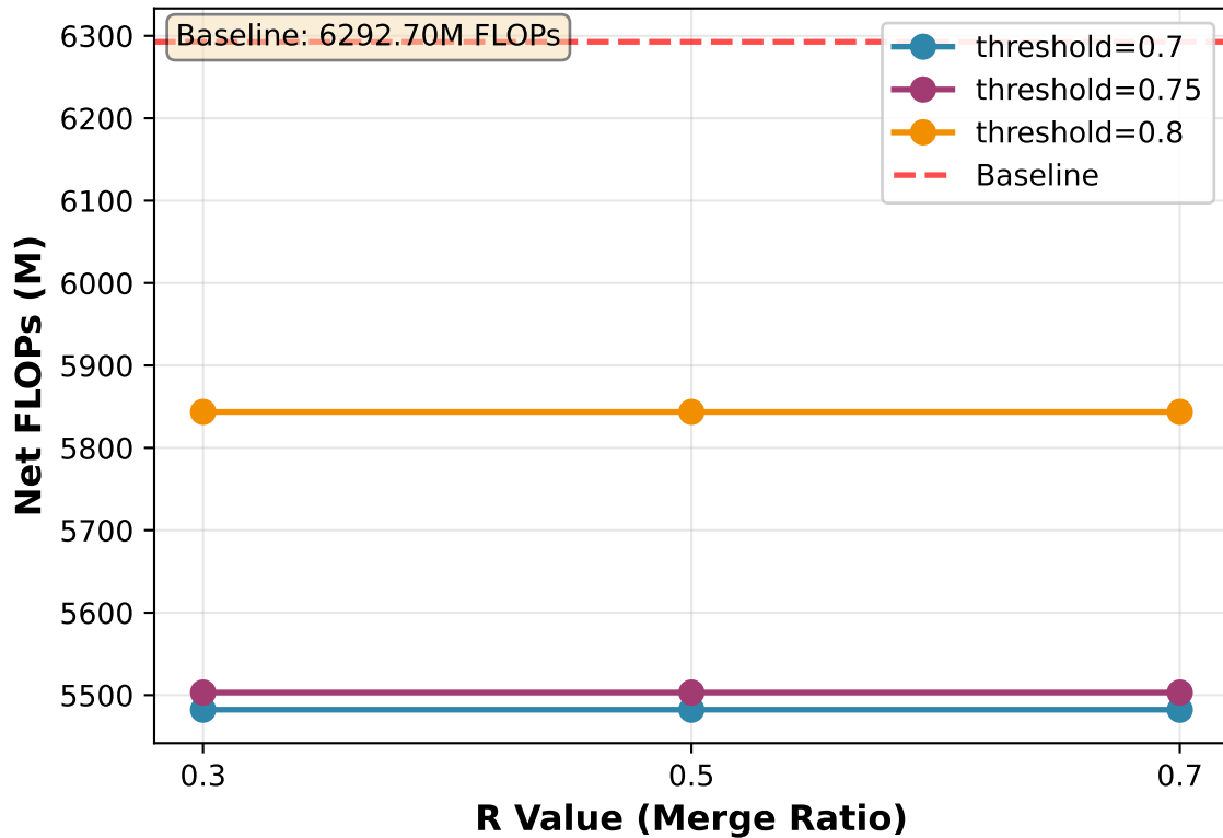
FLOPs vs R Value (saliency=4)
