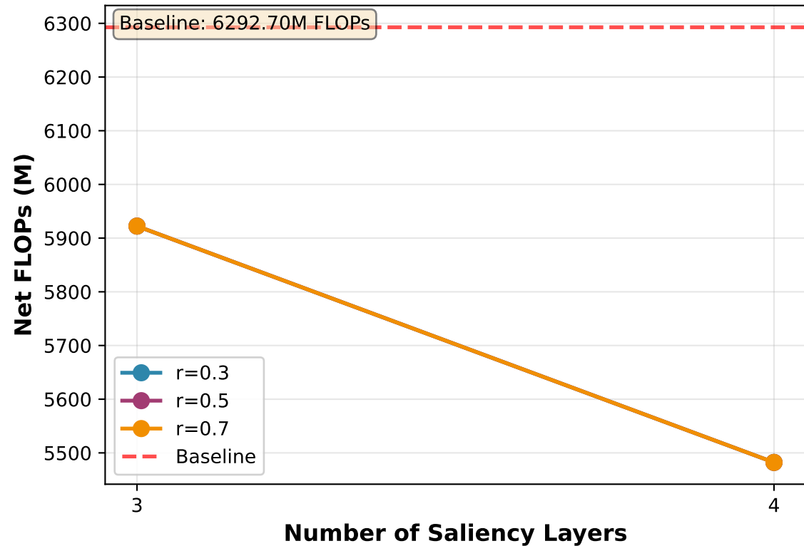
FLOPs vs Saliency Layers (threshold=0.70)
