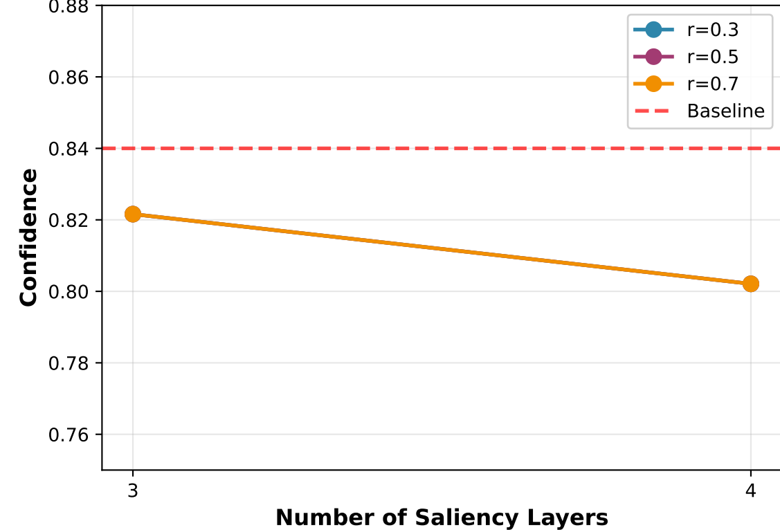
Confidence vs Saliency Layers (threshold=0.70)
