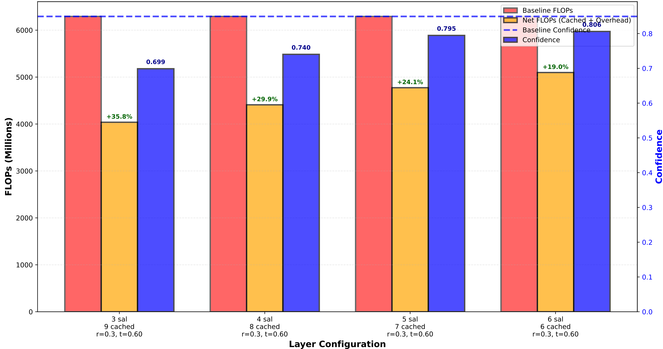
Best Configuration per Saliency Layer Count (maximizing FLOP reduction while maintaining confidence)
