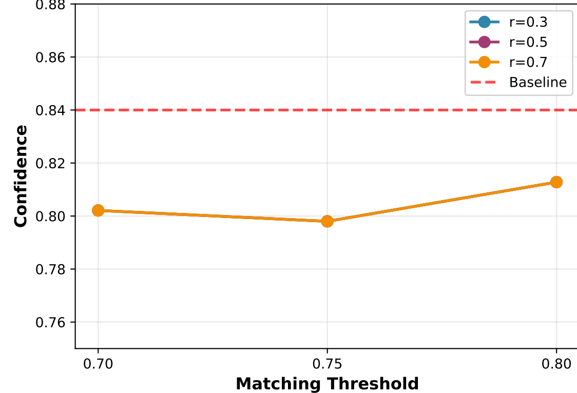
Confidence vs Threshold (saliency=4)
