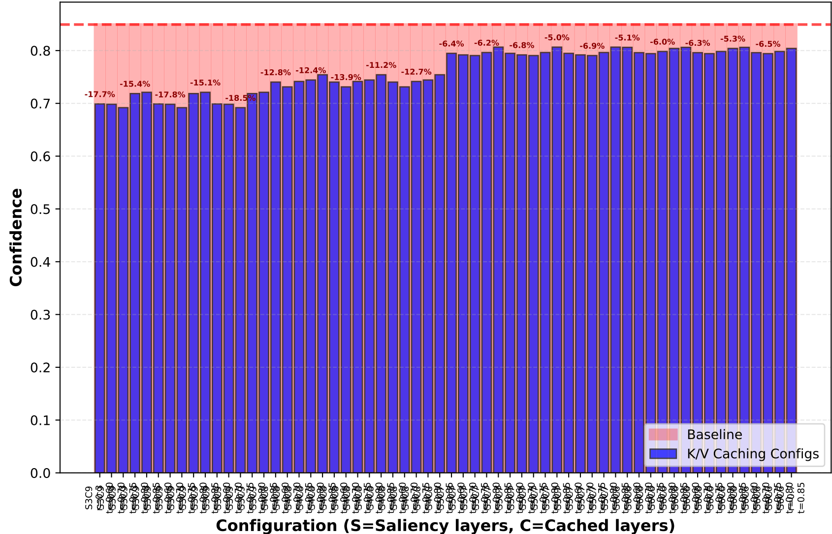
Confidence: Baseline vs All Configurations
