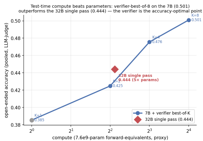
Fig. 6. Test-time compute beats parameters: 7B+verifier (0.501) > 32B single pass (0.444).
