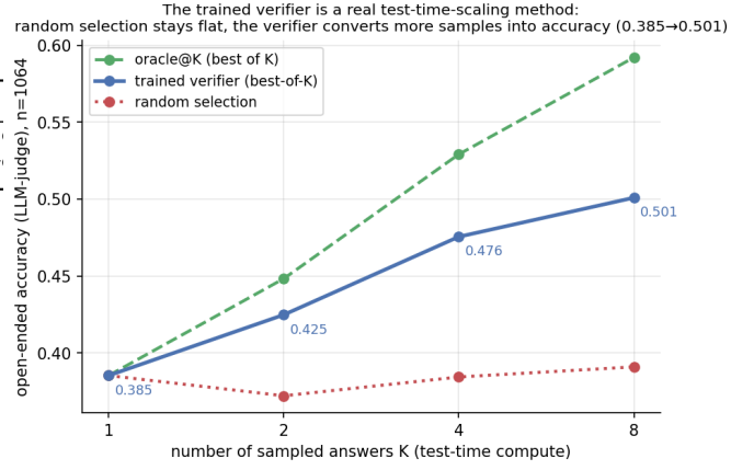
Fig. 4. Best-of- K : the trained verifier converts more samples into accuracy; random stays flat.
