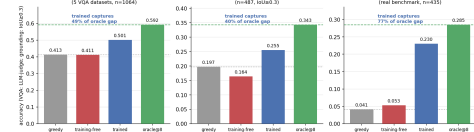
Fig. 5. Training breaks the luck floor across output types: free-text, SLAKE boxes, and real MS-CXR.
