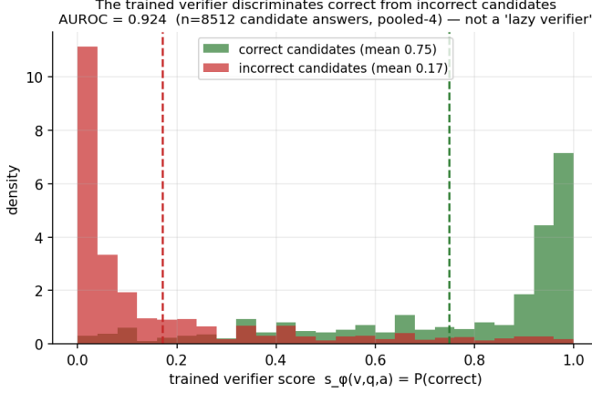
Fig. 3. The verifier separates correct from incorrect candidates (AUROC 0.924, n=8512 )—not a “lazy verifier.”
