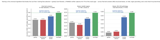
Fig. 5. Training breaks the luck floor across output types: free-text, SLAKE boxes, and real MS-CXR.
