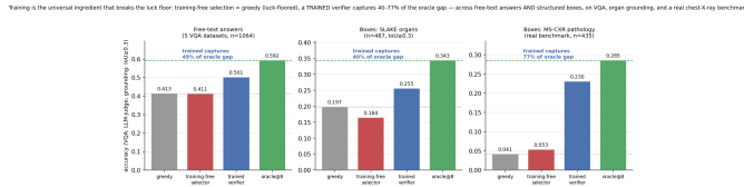
Fig. 5. Training breaks the luck floor across output types: free-text, SLAKE boxes, and real MS-CXR.
