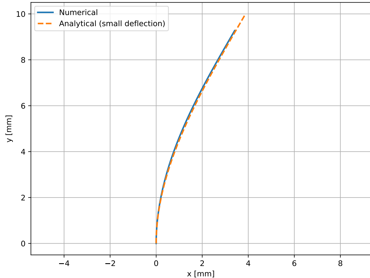
Shape of Cylinder under Magnetic Torque
