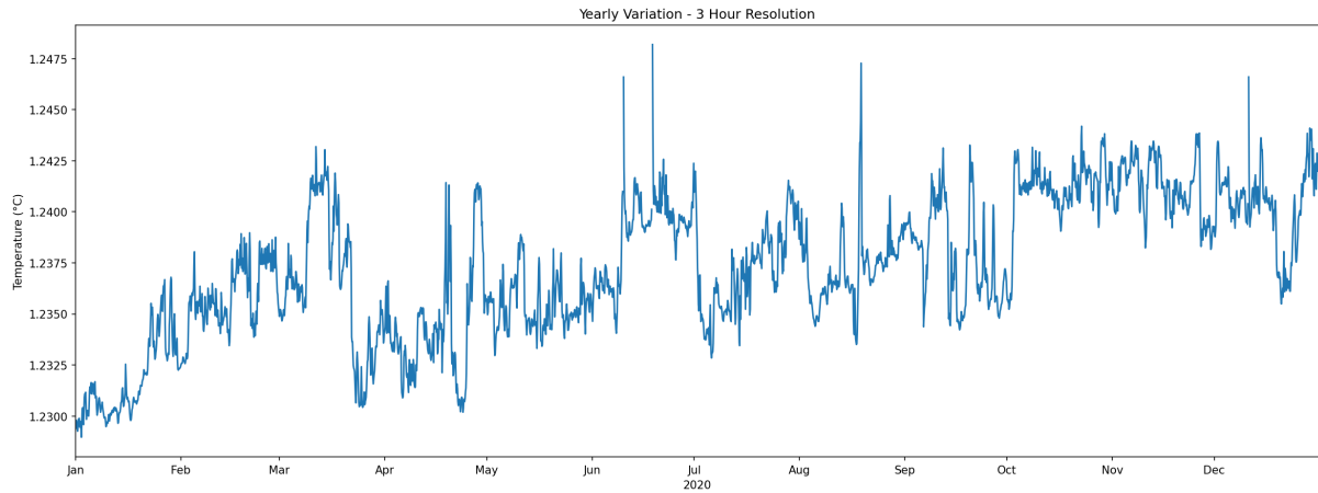
Figure 13 – 2020 yearly temperature with points grouped into 3-hour intervals, after removing readings above 1.25°C
