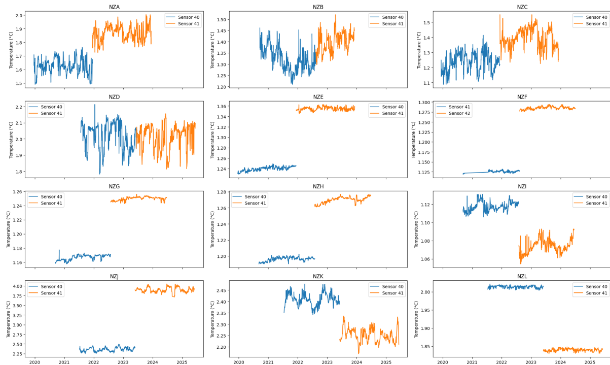
Figure 9 – Comparison of sensors at each station, with outliers removed using the 1.5 \times interquartile range rule
