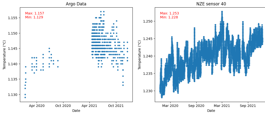
Figure 11 – Left is the Argo data, and right is the DART data with outliers removed. The maximum and minimum range is in the top left of each graph
