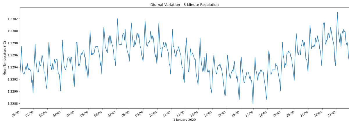
Figure 12 – The daily temperature on 1 January 2020 with points grouped into 3-minute intervals
