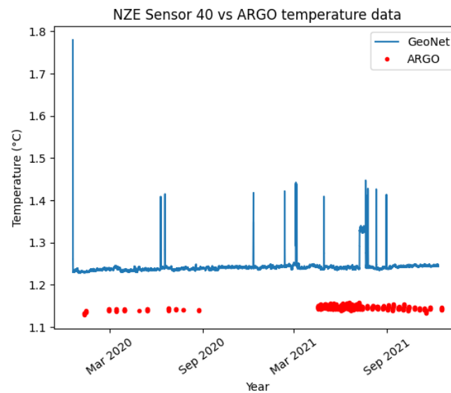
Figure 10 – Argo temperature data in red and DART (GeoNet) temperature data in blue
