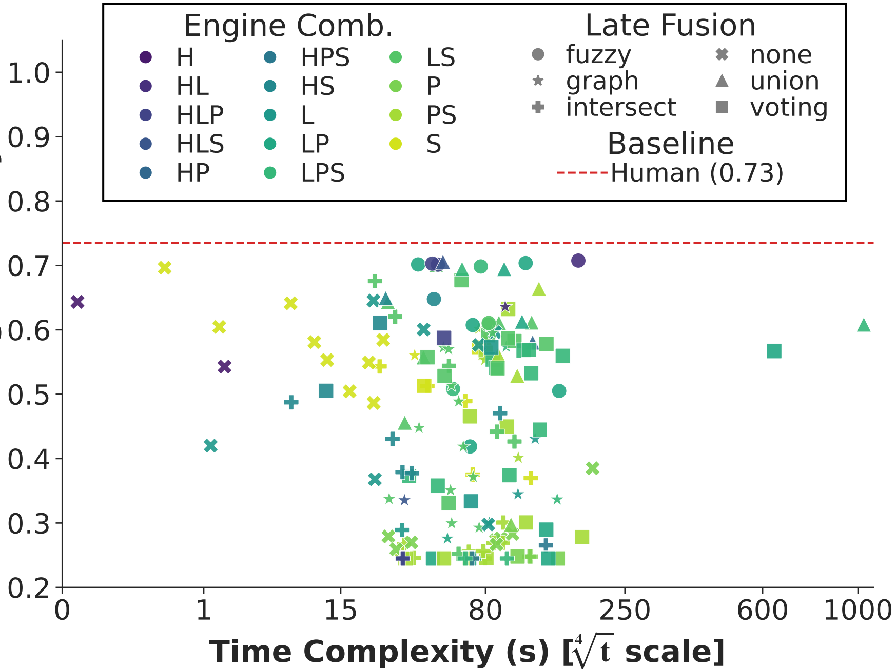
Bounding Similarity
