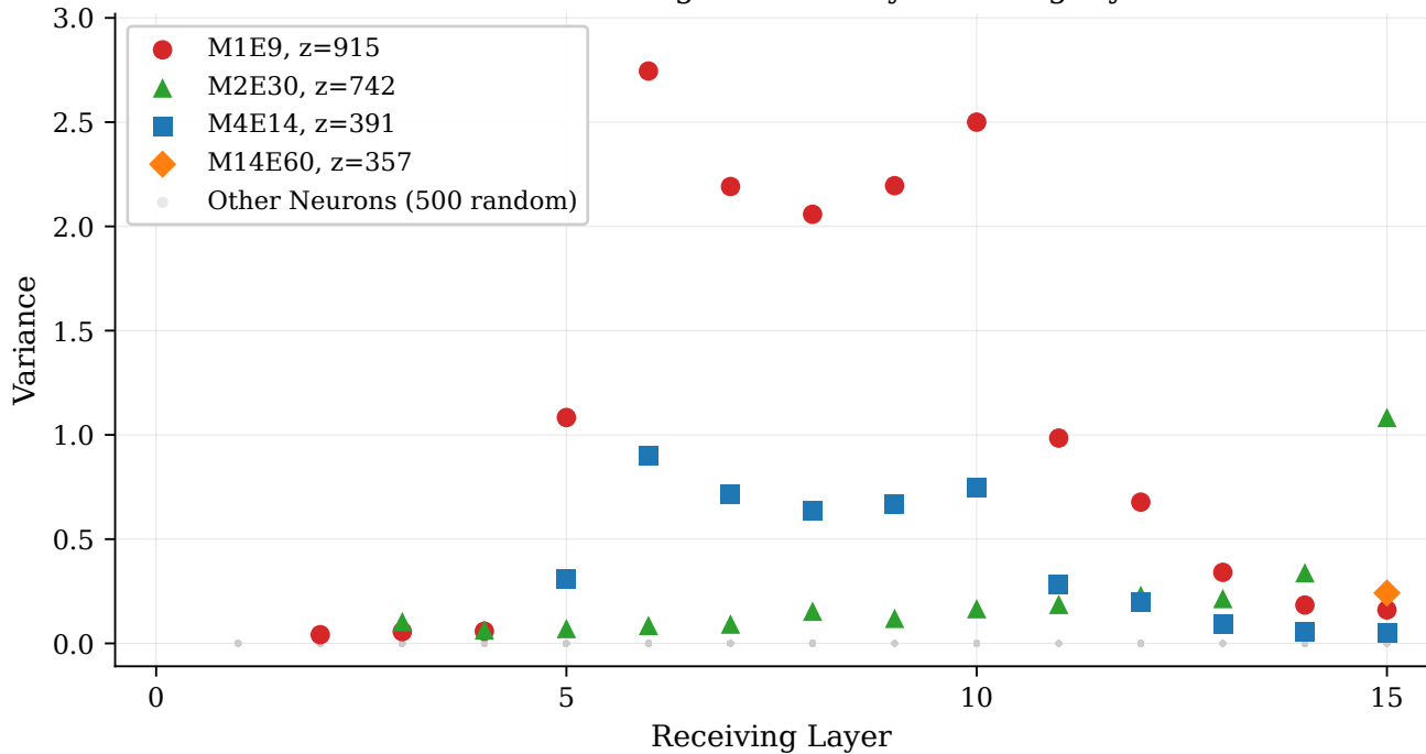
Per-neuron routing influence by receiving layer
