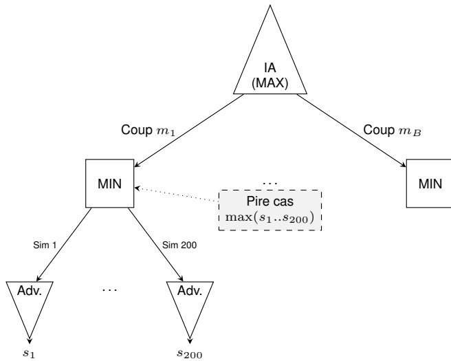
FIGURE 3 – Agrégation Pessimiste
