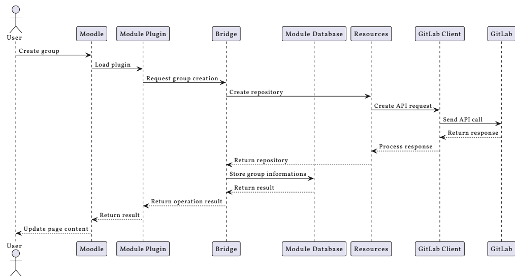
Figure 8: Components interactions during group creation
