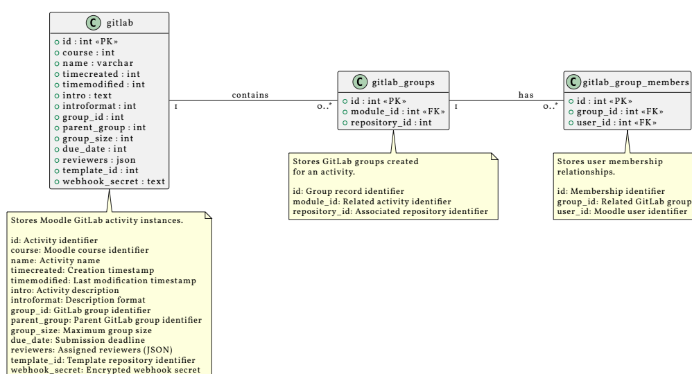
Figure 19: Module plugin database schema
