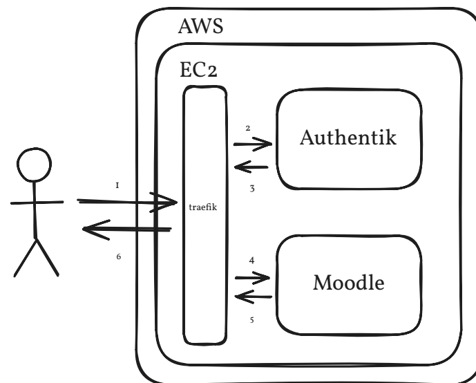
Figure 17: IaC architecture
