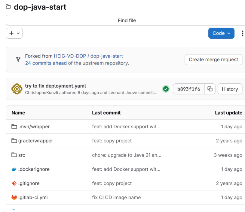
Figure 2: GitLab repository
