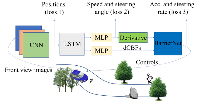
Fig. 12. Multilevel interpretable end-to-end autonomous driving framework with dCBFs. The entire pipeline is end-to-end differentiable. Each depth of the model learns different vehicle and environment information. The outputs of BarrierNet are high-relative-degree controls.
