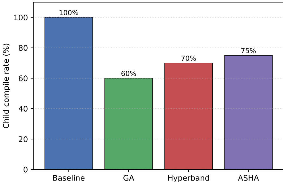
Compile reliability of generated children
