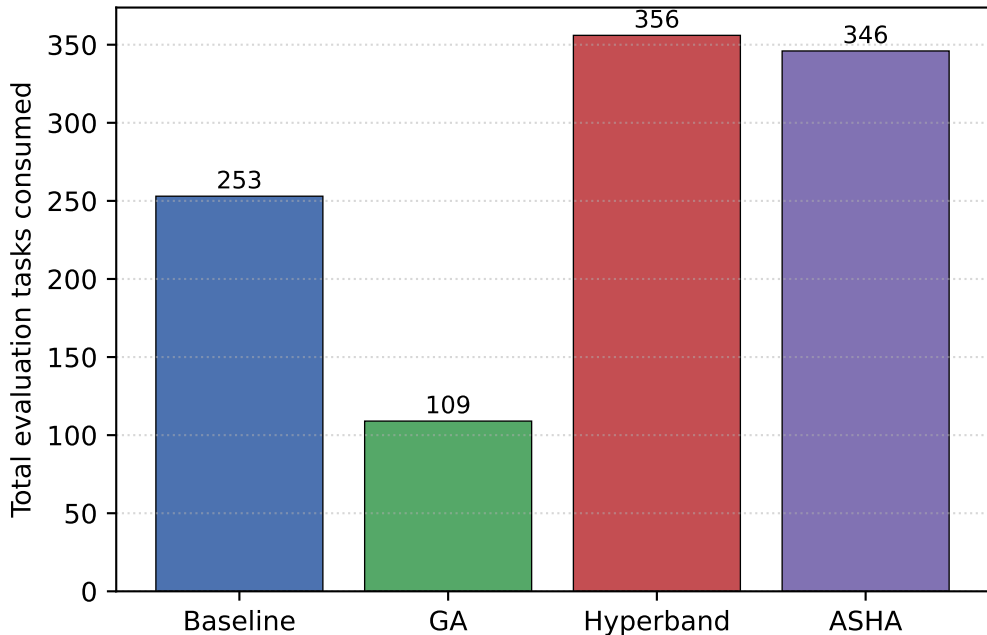
Evaluation-budget consumption (4 generations)
