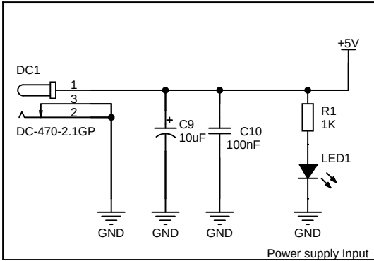
Power supply Input
