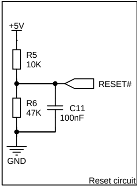
Reset circuit
