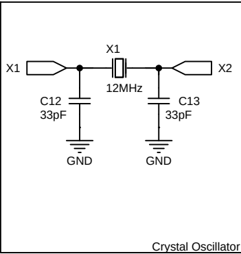
Crystal Oscillator
