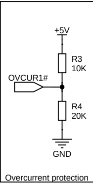
Overcurrent protection
