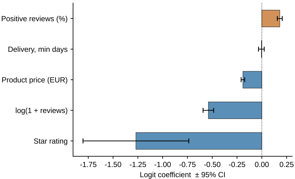
Coefficient estimates
