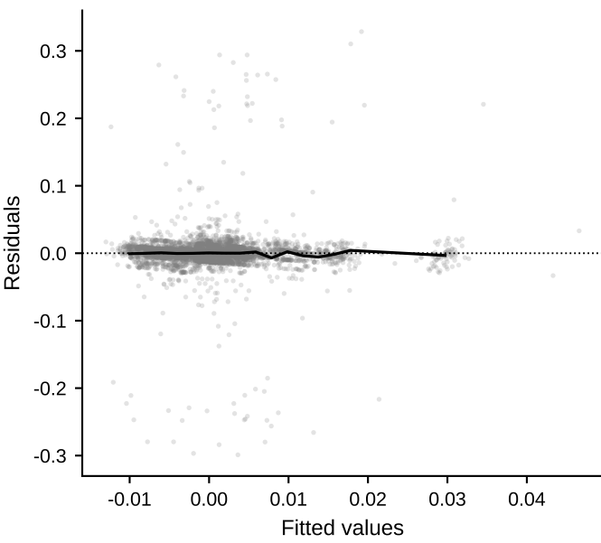
D1 dynamic OLS (n = 4,958; seller and transition FE)
