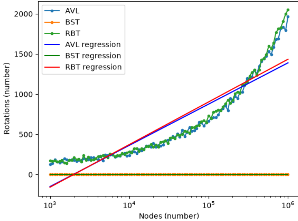
Figure 7: AVL, BST and RBT rotation in logarithmic scale and with logarithmic regression functions
