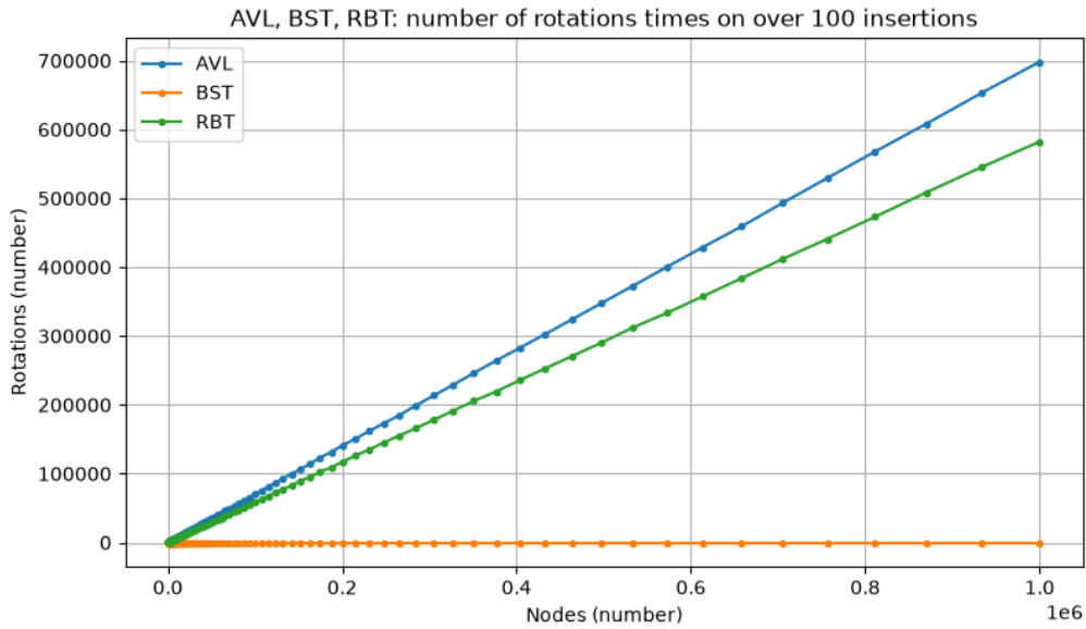
Figure 4: AVL rotation test
