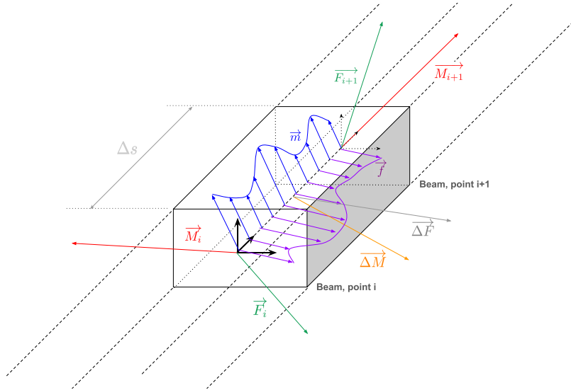
Figure 1.6: Beam element between position i and i + 1 . The scheme includes structural forces and moments at position i ( \vec{F}_i, \vec{M}_i ) and i + 1 ( \vec{F}_{i+1}, \vec{M}_{i+1} ), the distributed forces and moments ( \vec{f}, \vec{m} ) and concentrated forces and moments ( \Delta\vec{F}, \Delta\vec{M} )
