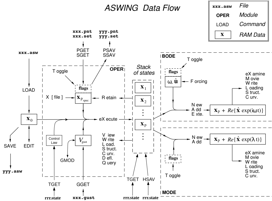
Figure 1.13: Schematic of ASWING typical pipeline [2]
