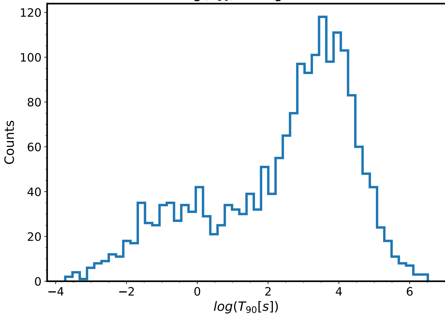
\log(T_{90}) histogram
