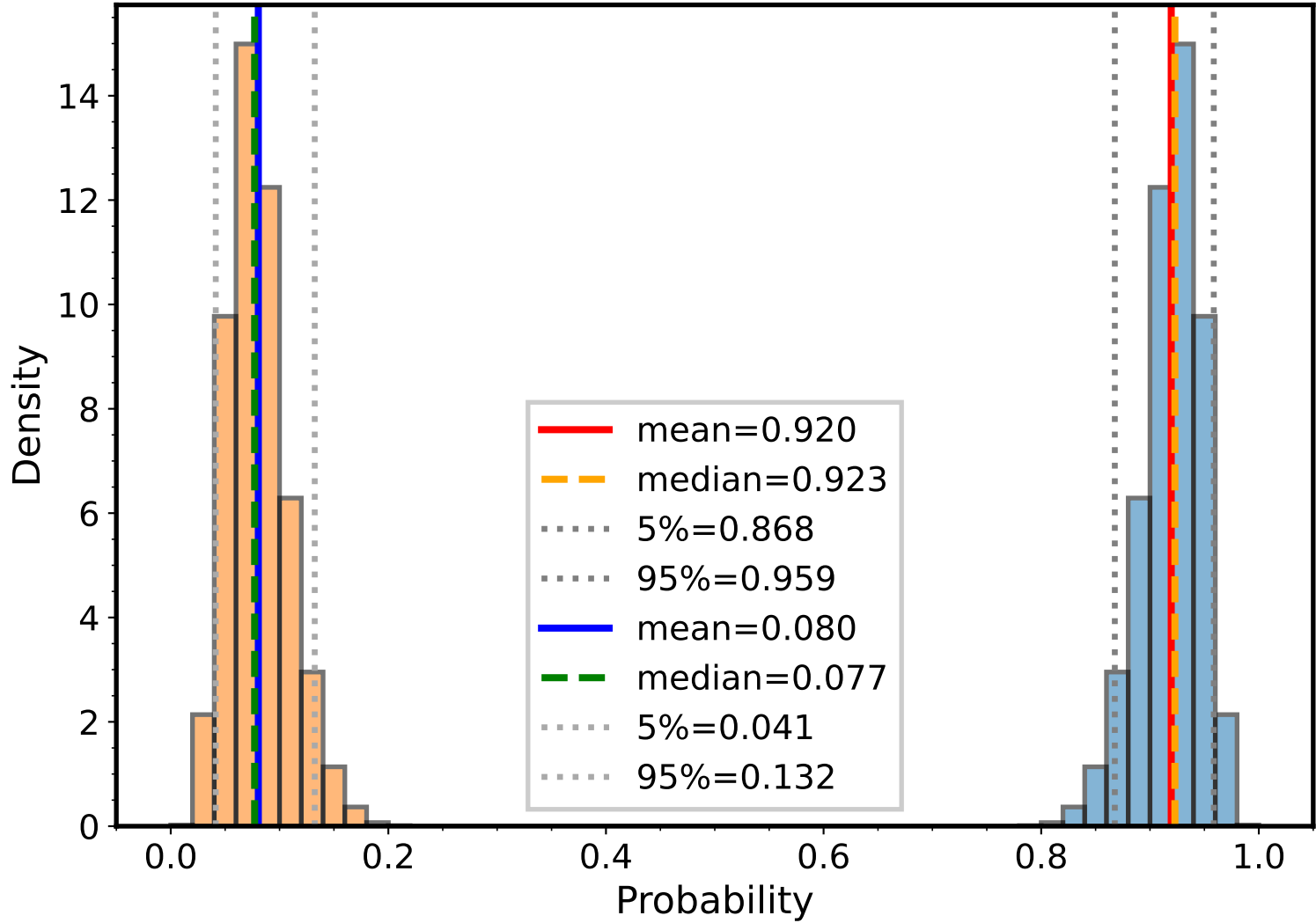
Histogram of P(\text{short} | x_{obs}, \theta) and P(\text{long} | x_{obs}, \theta) for x=\ln(2) ( x=0.693 )
