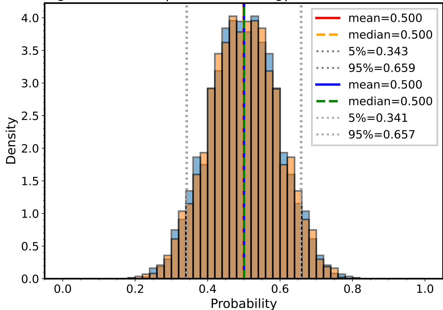
Histogram of P(\text{short} | x, \theta) and P(\text{long} | x, \theta) for x=\text{thr} ( x=1.585 )
