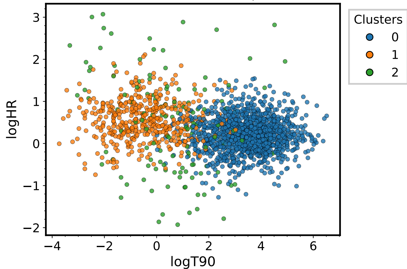
T90-HR clusters - \alpha=0.01 , \kappa_0=0.01
