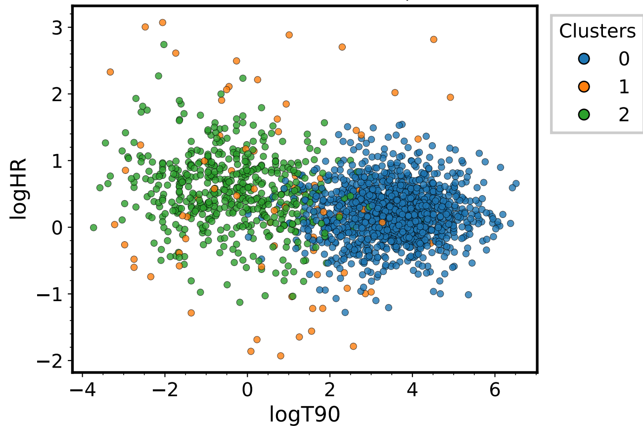
T90-HR clusters - \alpha=0.01 , \kappa_0=0.1
