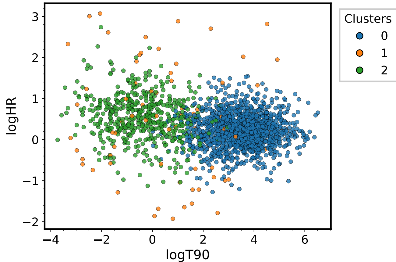
T90-HR clusters - \alpha=0.1 , \kappa_0=0.01
