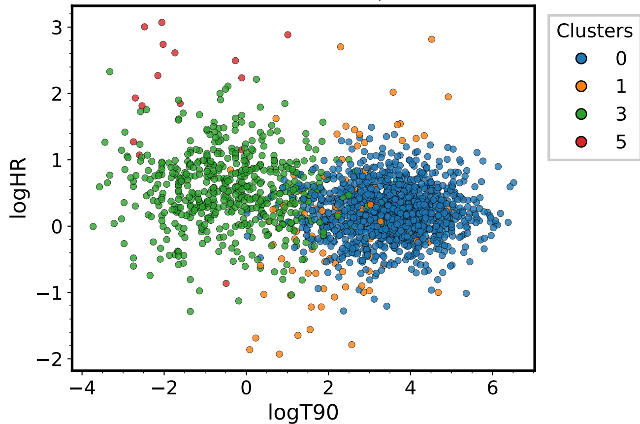
T90-HR clusters - \alpha=1 , \kappa_0=0.01
