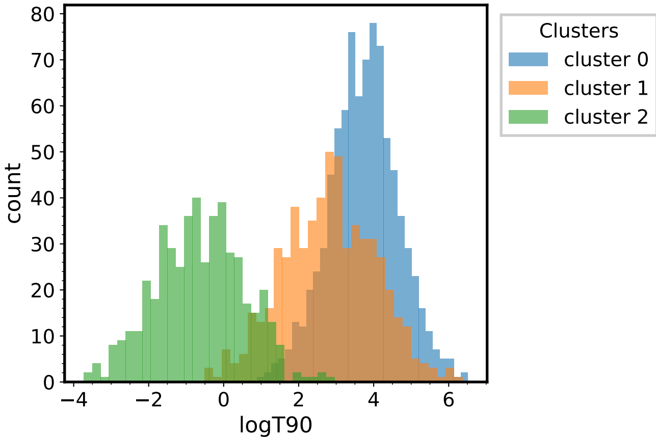
T90 clusters - \alpha=1e-10 , \kappa_0=0.01
