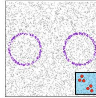
Unit Cube (no bound)
