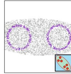
Single Ellipsoid
