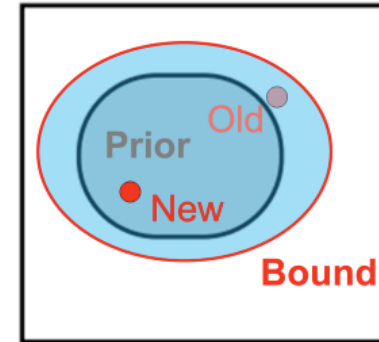
Uniform
