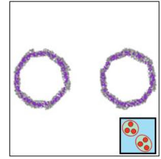
Multiple Ellipsoids
