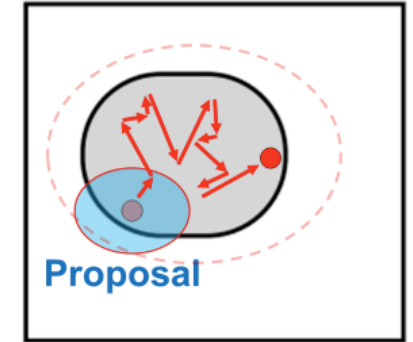
Random Walk
