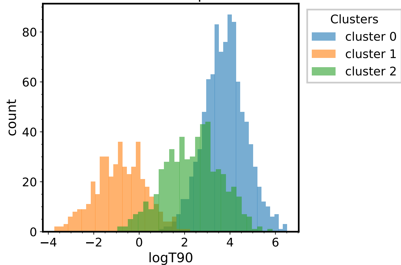
T90 clusters - \alpha=0.1
