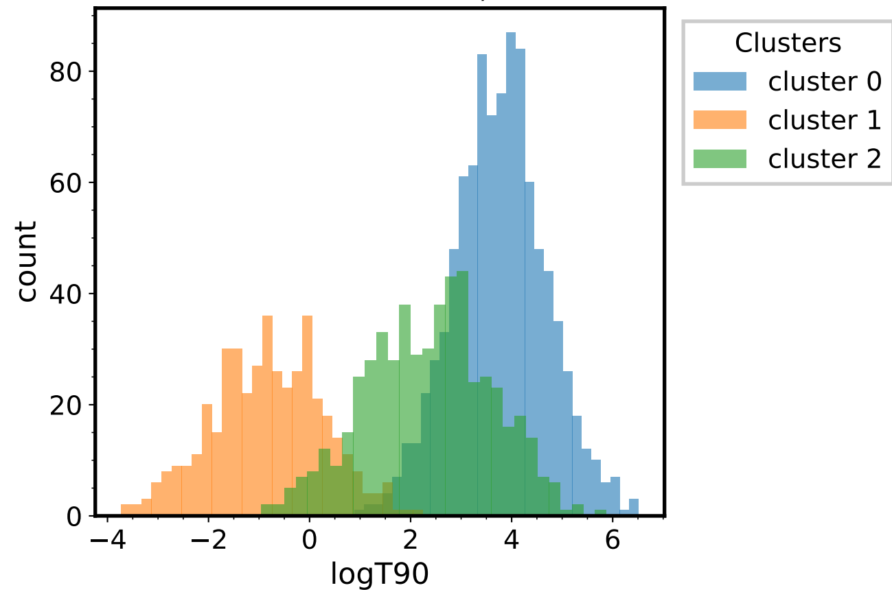
T90 clusters - \alpha=0.1 , \kappa_0=0.1
