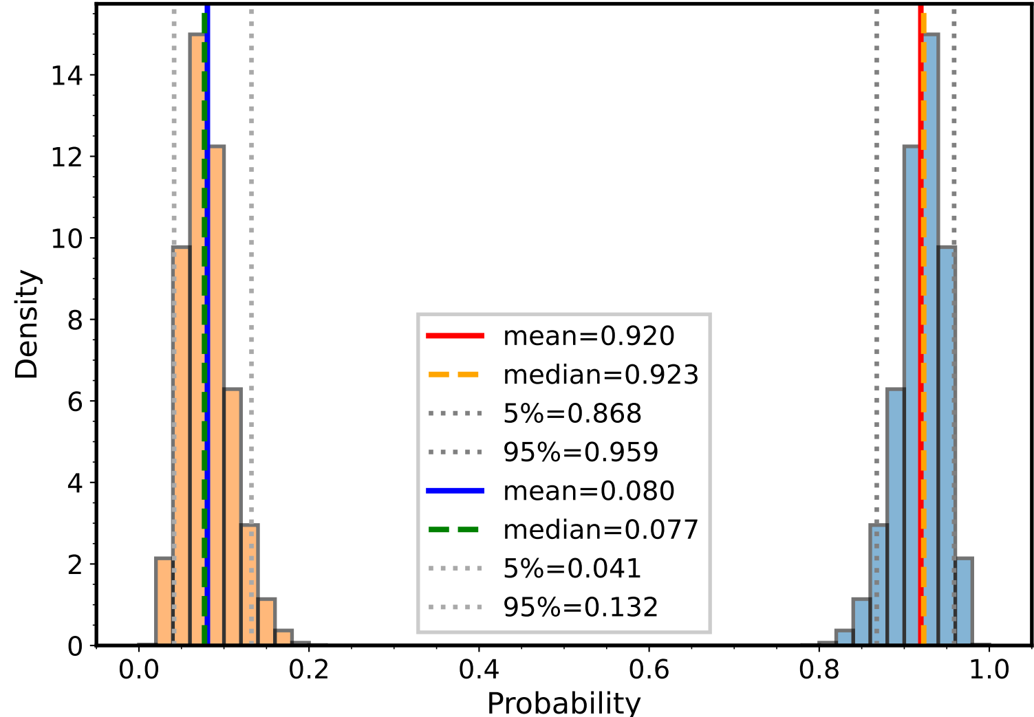
Histogram of P(\text{short} \mid x_{\text{obs}}, \theta) and P(\text{long} \mid x_{\text{obs}}, \theta) for x=\ln(2) ( x=0.693 )
