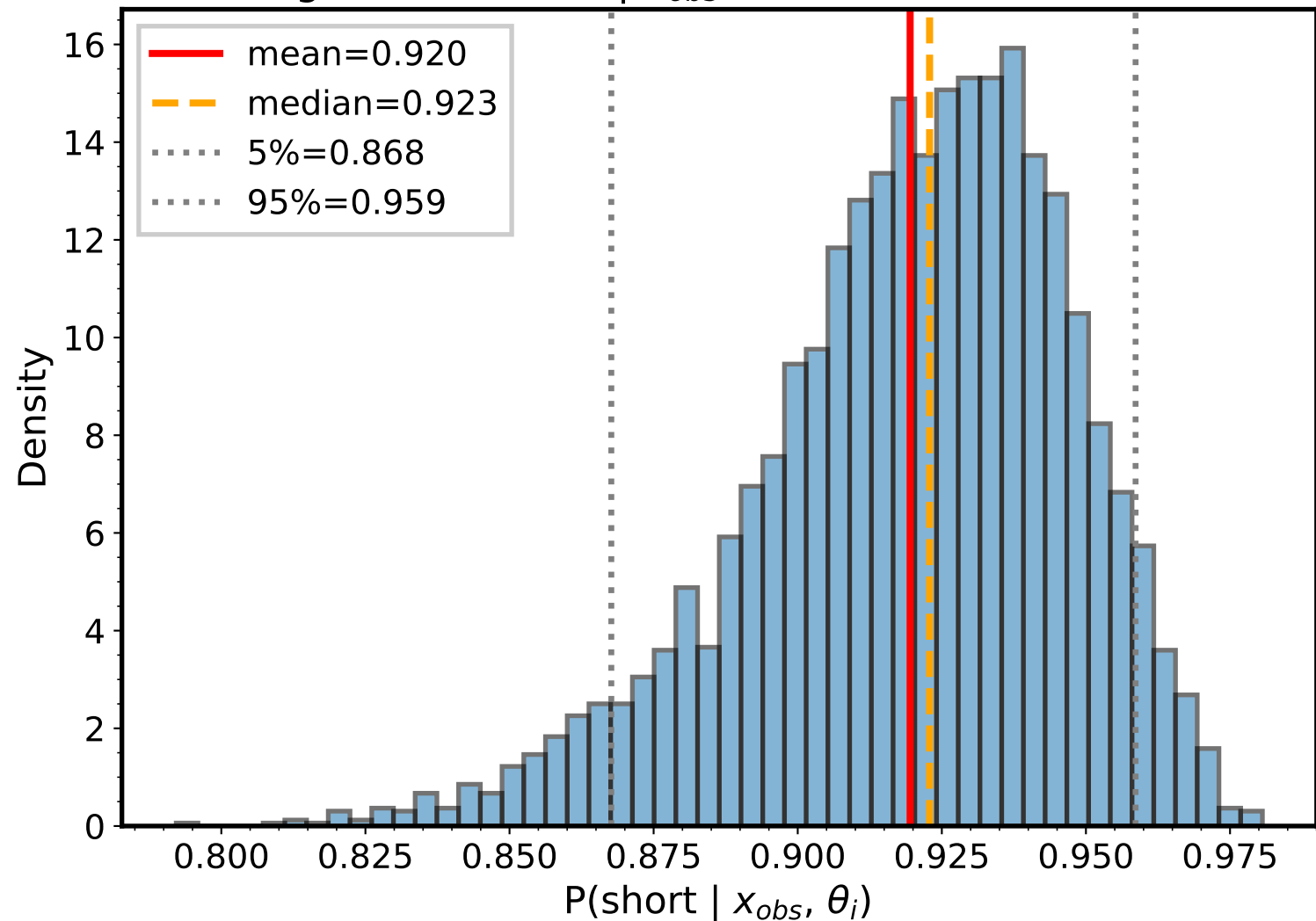
Histogram of P(\text{short} | x_{obs}, \theta) for x=\ln(2) ( x=0.693 )
