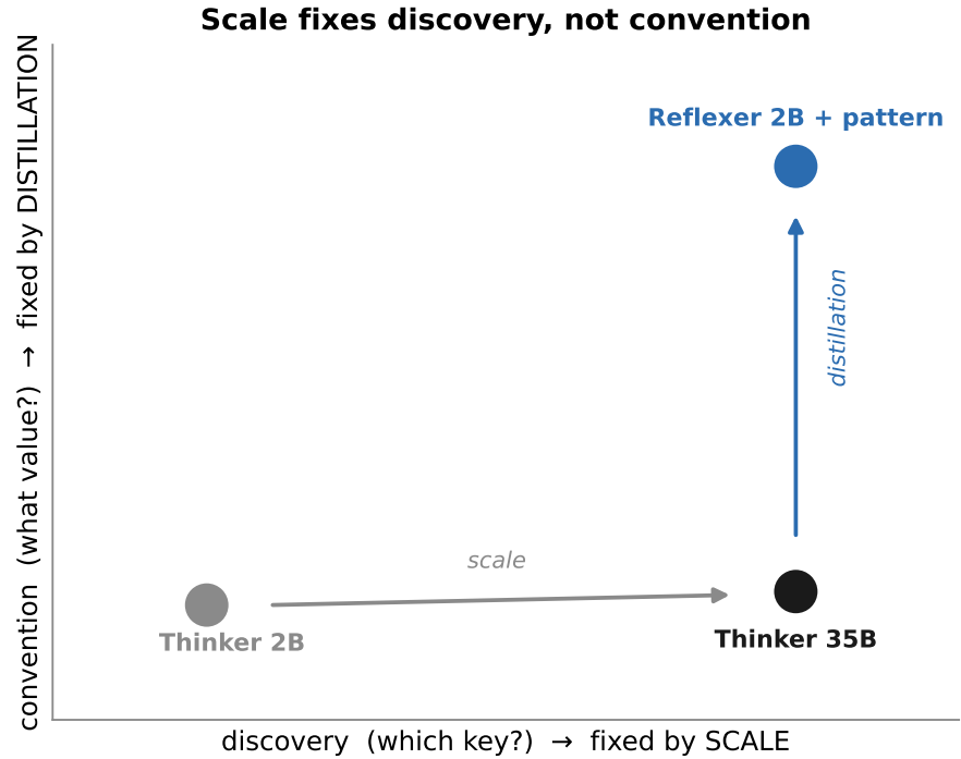
Figure 5.3: Why a distilled pattern beats a 17\times larger model on the realistic API: the bottleneck is undiscoverable convention, not reasoning.
