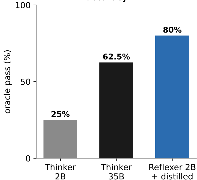
SET-2 realistic API accuracy win
