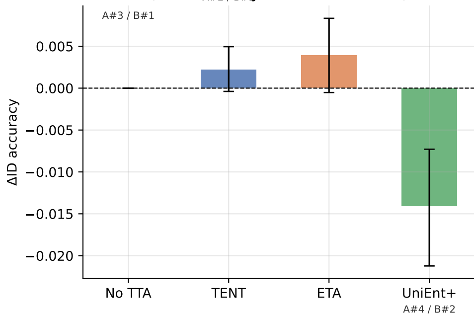
Panel A — Closed-Set Ranking ( \Delta ID accuracy, no OOD in batch)
