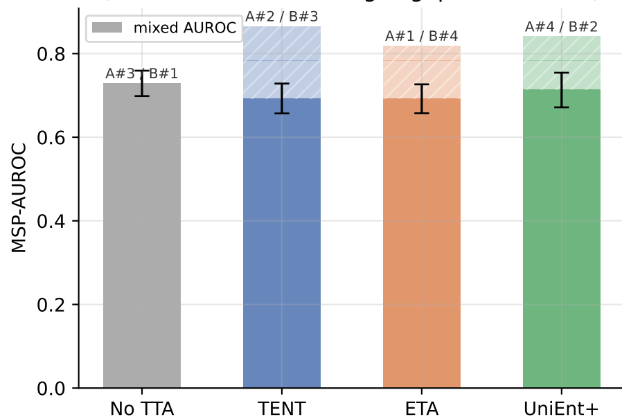
Panel B — Open-World Safety Ranking (mixed AUROC; hatching = gap to ID-Oracle)
