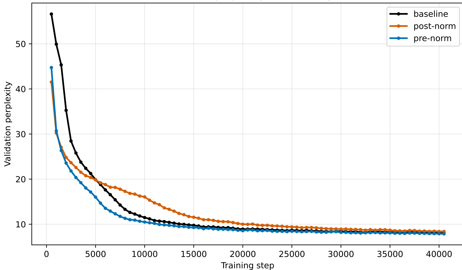
Validation perplexity over training
