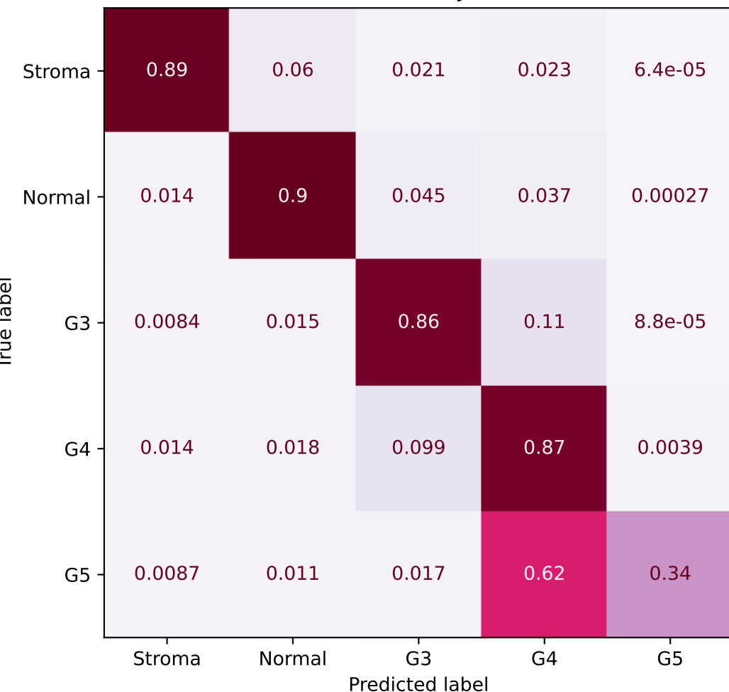
Confusion matrix using OT_multi_no_detach for KFBio_FDA balanced accuracy = 77.35%
